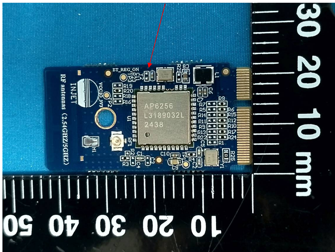
Fixture board
