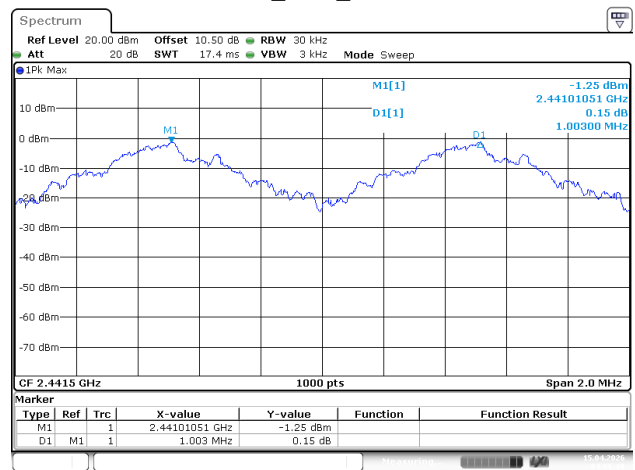
BDR_DH1_Middle
