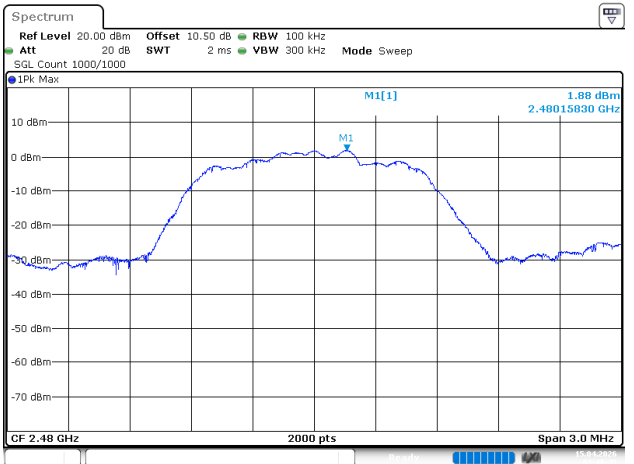
3EDR_DH1_High
