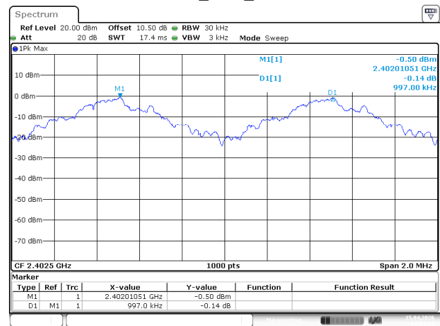
BDR_DH1_Low
