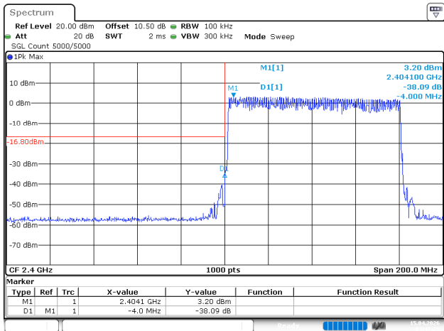
3EDR_DH1_Hopping_Lower
