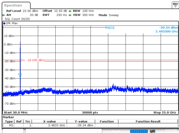
2EDR_DH1_High
