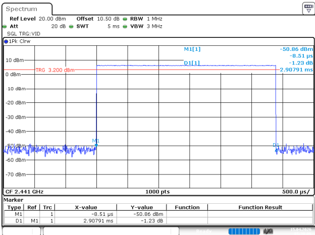
BDR_DH5_Hopping
