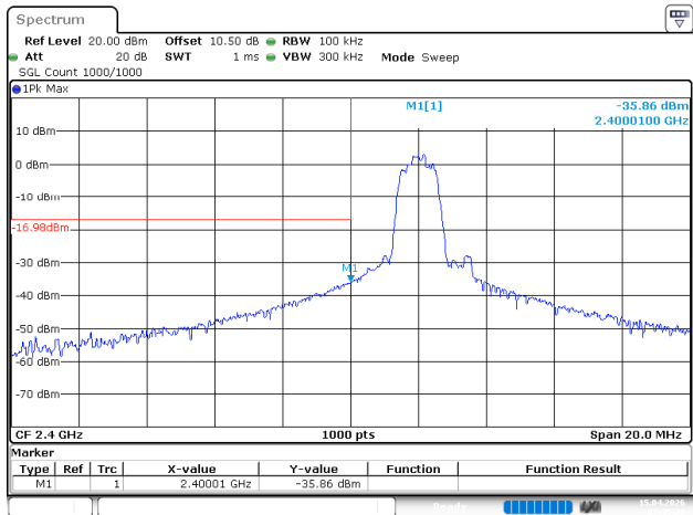
3EDR_DH1_Low
