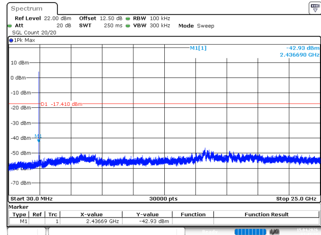
3EDR_DH1_Middle
