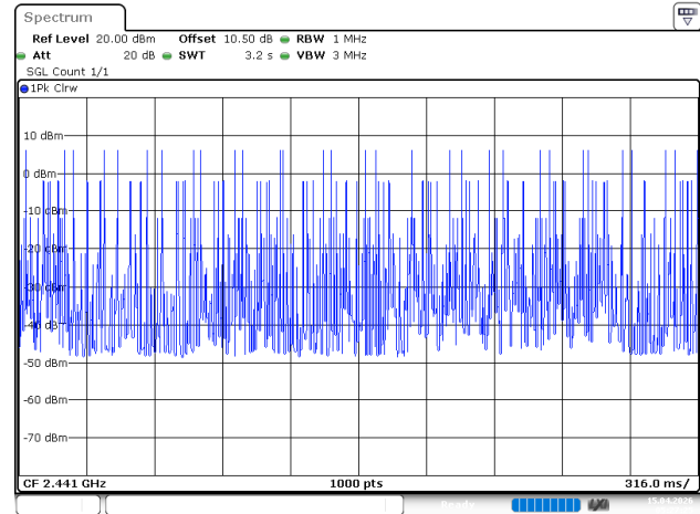
BDR_DH1_Hopping
