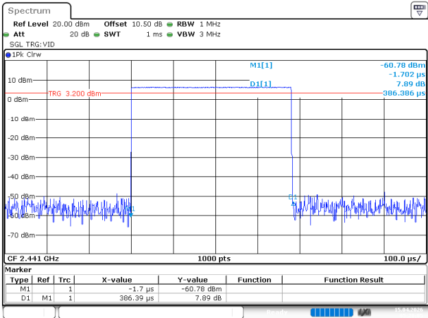
BDR_DH1_Hopping
