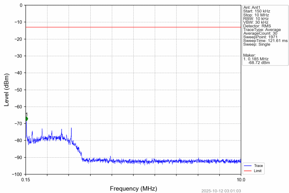
Band66_3MHz_16QAM_MCH_1745MHz_RB_1_0_NTNV
