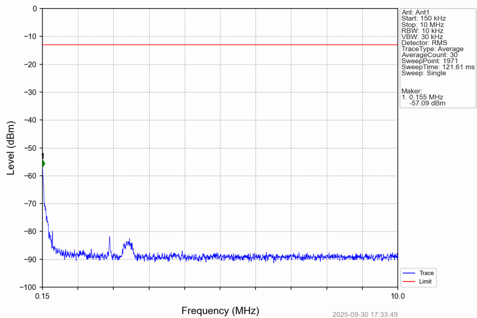
Band12_3MHz_16QAM_MCH_707.5MHz_RB_1_0_NTNV
