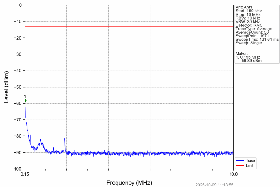
Band66_1.4MHz_QPSK_HCH_1779.3MHz_RB_1_0_NTNV
