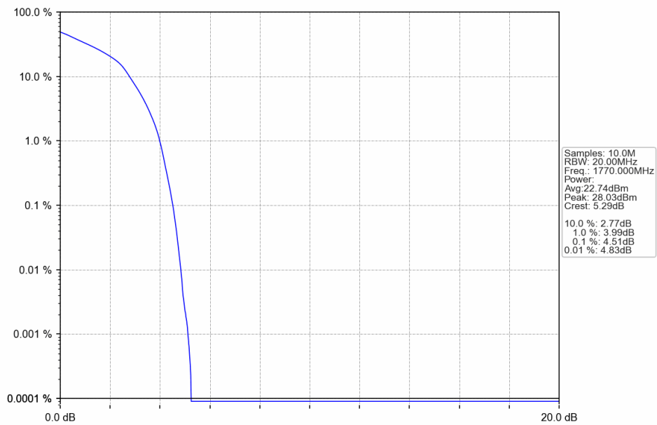
Band66_20MHz_16QAM_HCH_1770MHz_RB_27_73_NTNV
