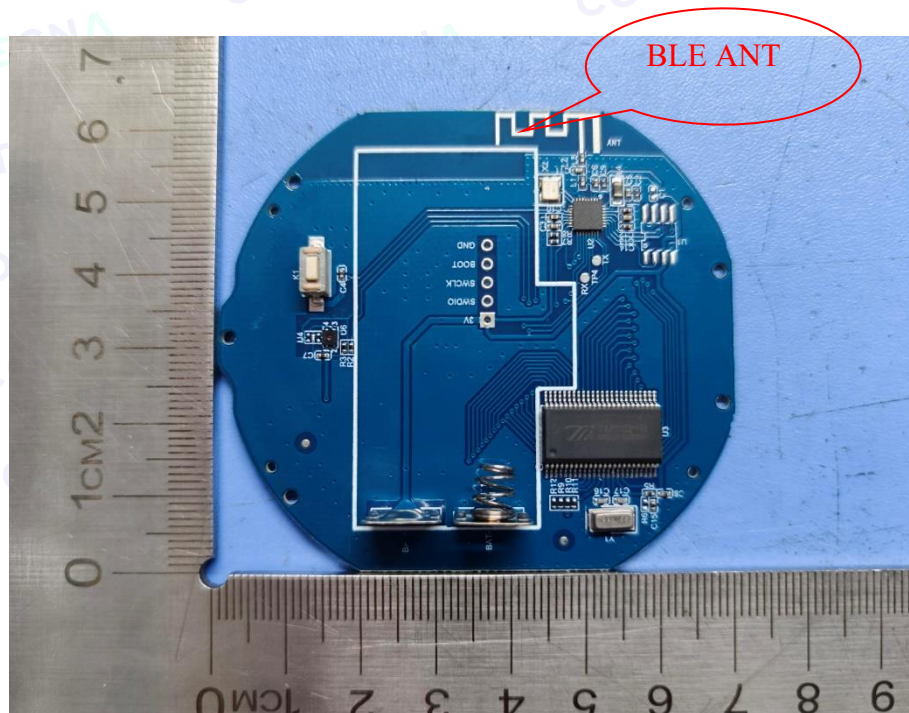
Photo 10 Appearance of PCB
