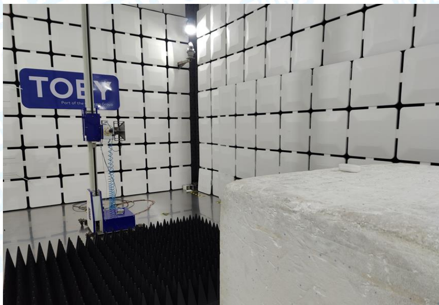
Photo of Setup for Radiated Emission (Above 1 GHz)
