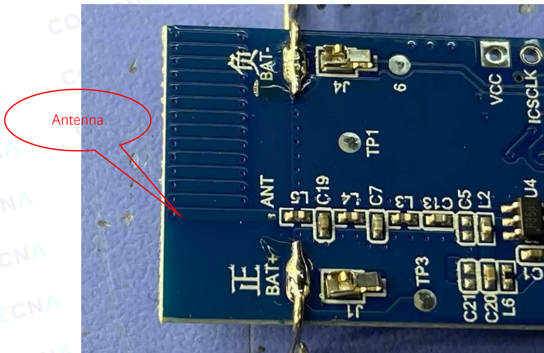
Photo 12 Appearance of PCB
