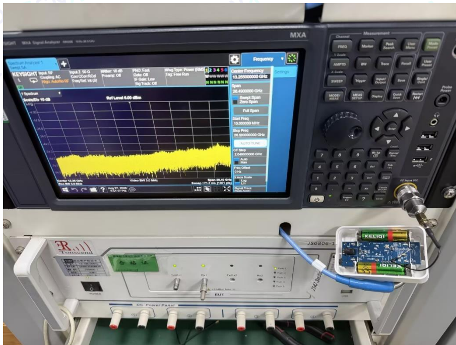
Photo of Setup for RF Conducted
