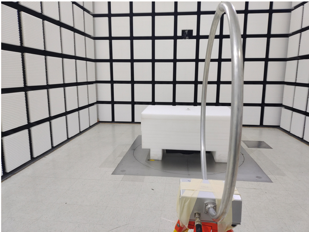
Radiated Emission 9kHz to 30MHz Perpendicular
