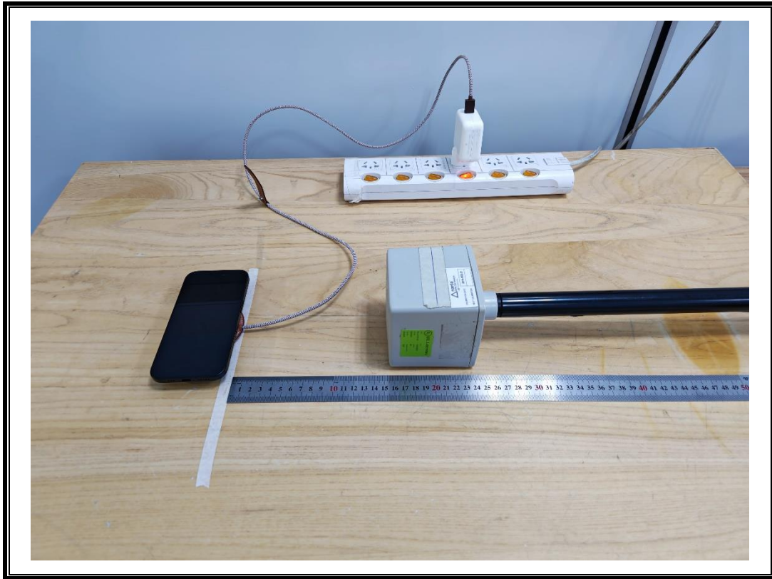
E-FILED AND H-FILED STRENGTH MEASUREMENT SETUP-2
