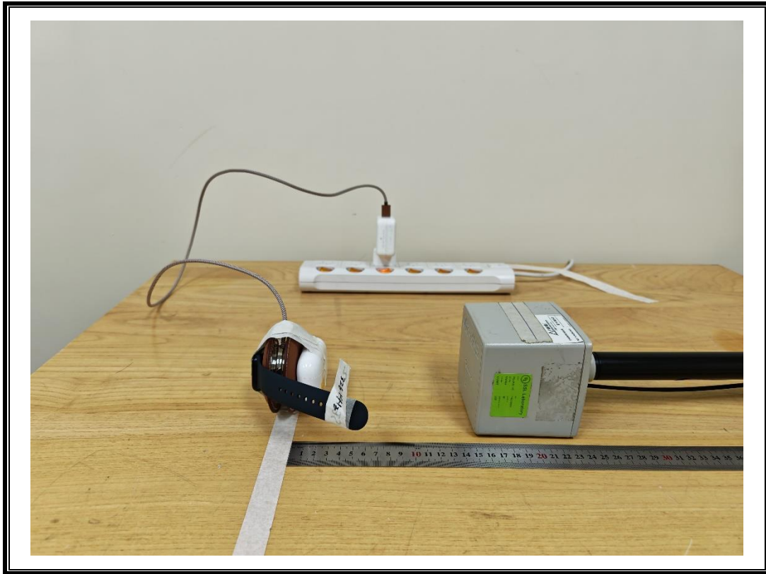
E-FILED AND H-FILED STRENGTH MEASUREMENT SETUP-6
