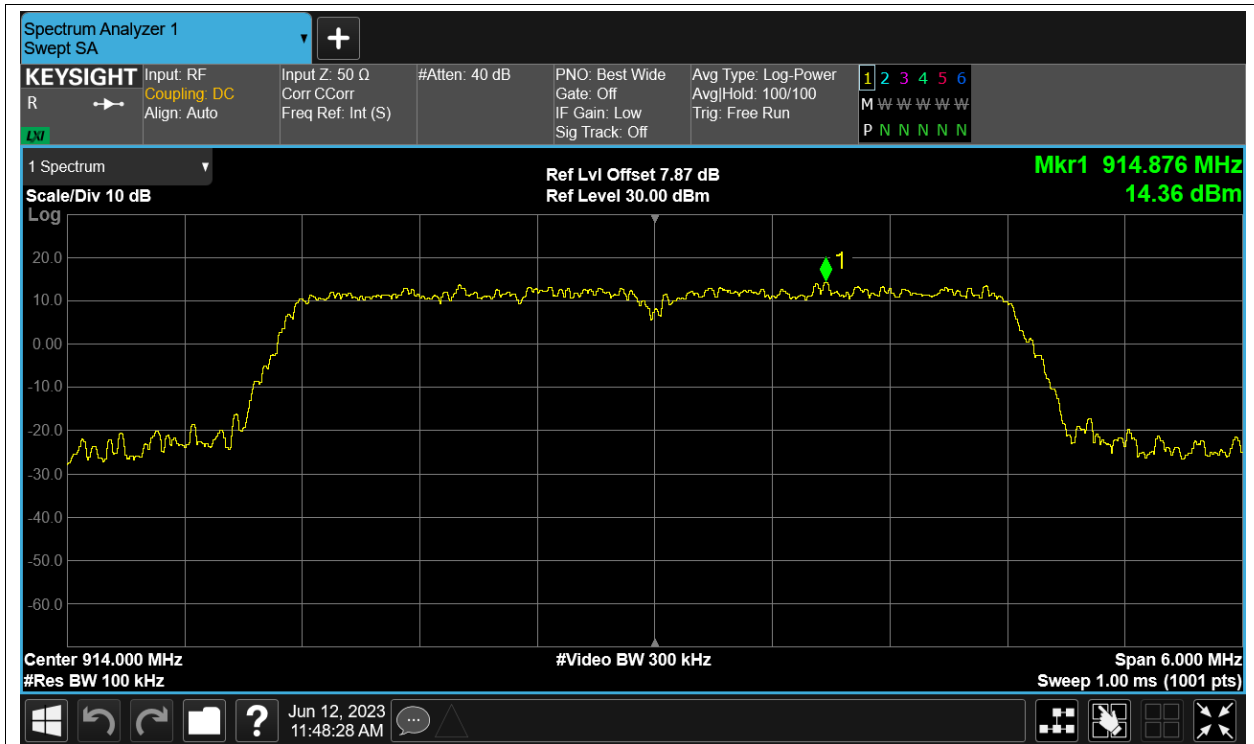
Tx. Spurious NVNT AH 914MHz Ant1 Emission
