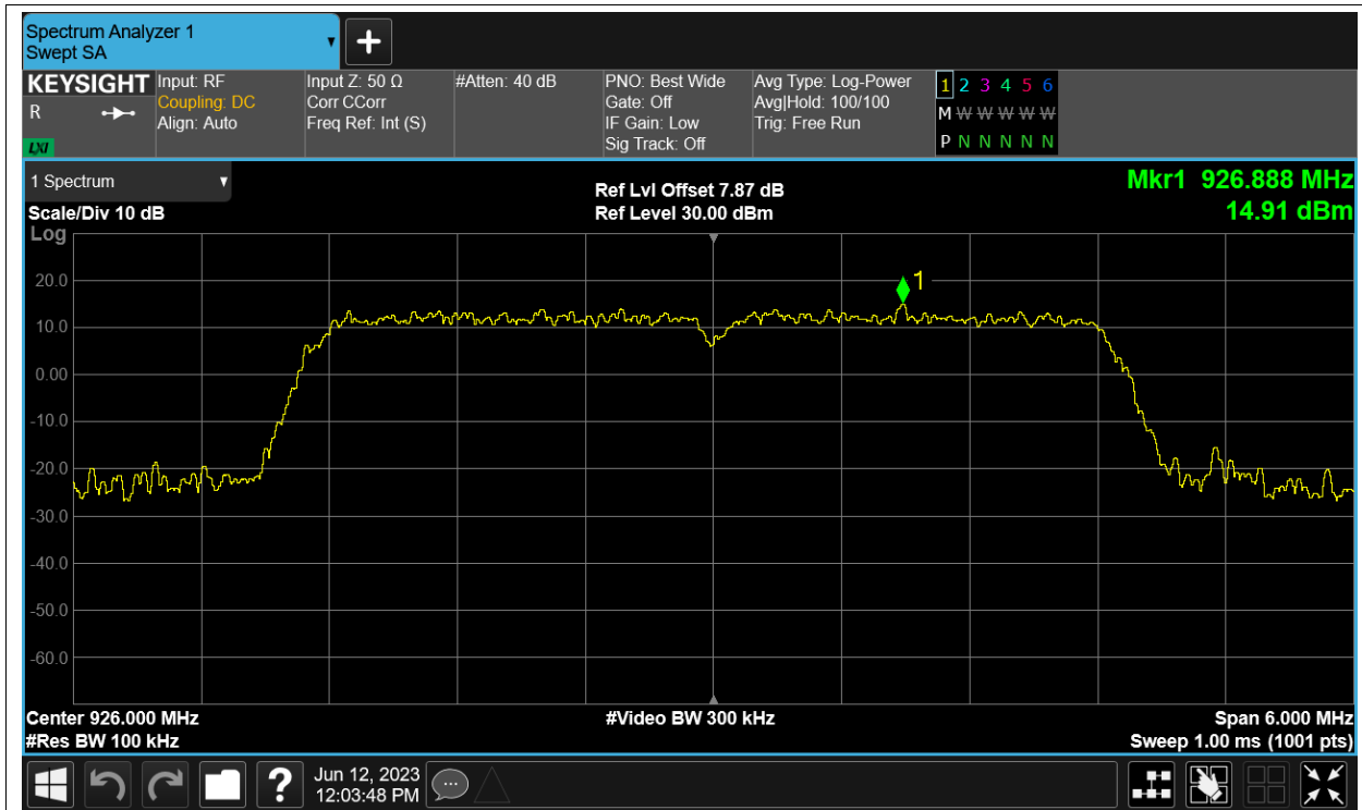
Band Edge NVNT AH 926MHz Ant1 Emission
