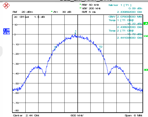
BLE_2M_Ant1_2440
