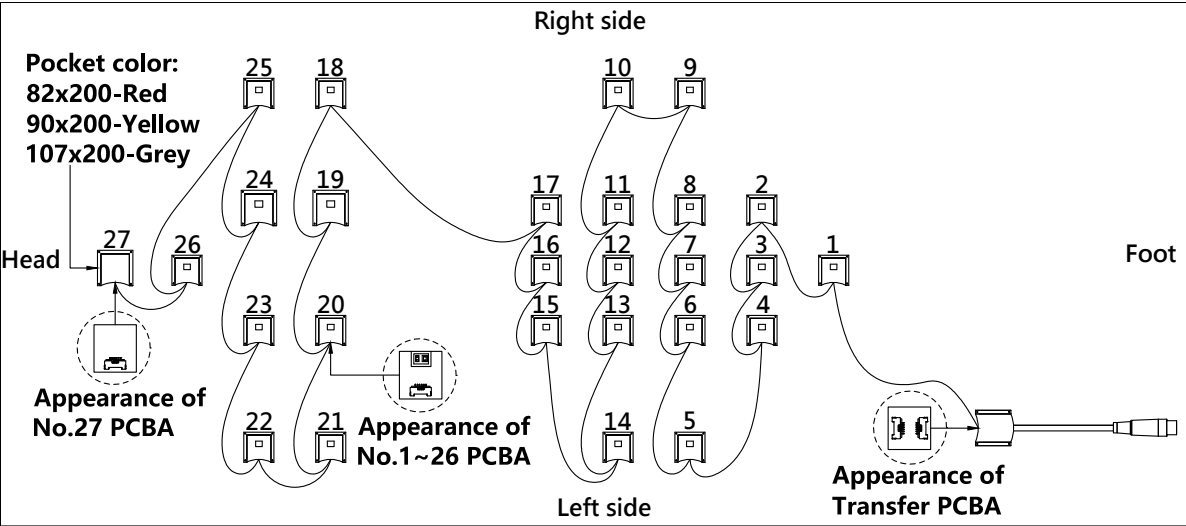
Sensor Pad Assembly Configuration Drawing (Back View):
