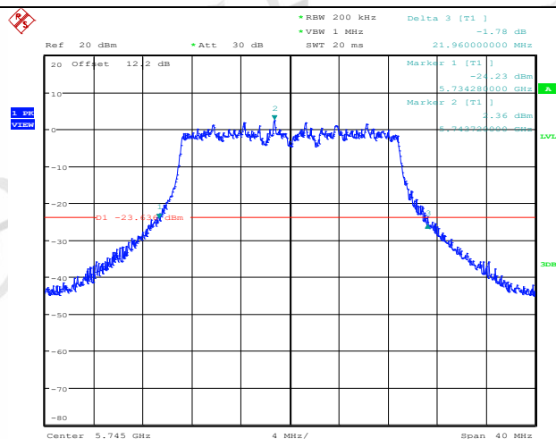
20 MHZ Ant2 5745
