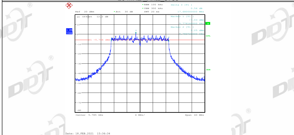
20 MHz_Ant2_5785
