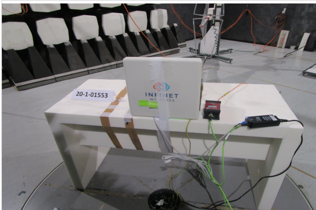
Photograph 1: EUT Test Setup in the semi anechoic chamber, Electric Field Strength
