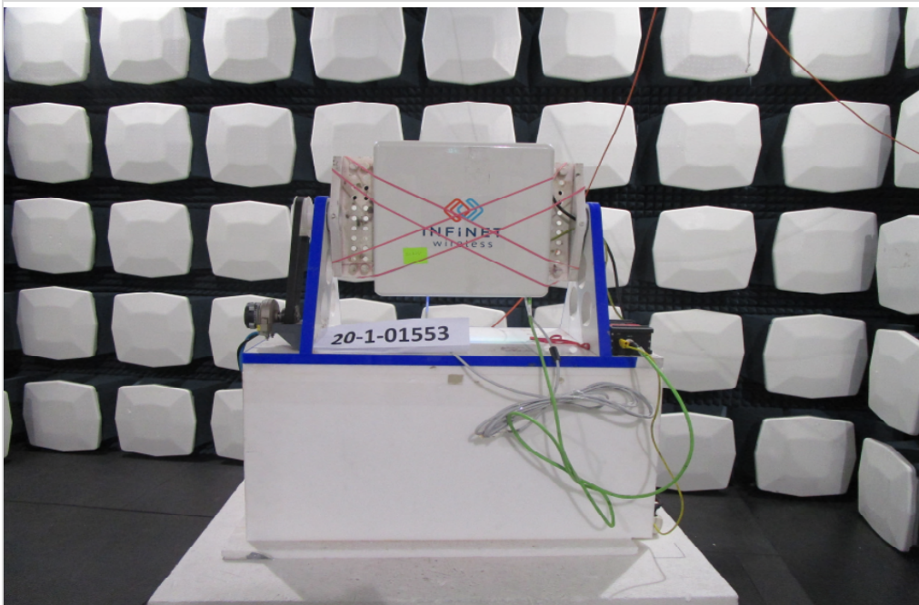
Photograph 3: EUT Test Setup in the fully anechoic chamber, Electric Field Strength
