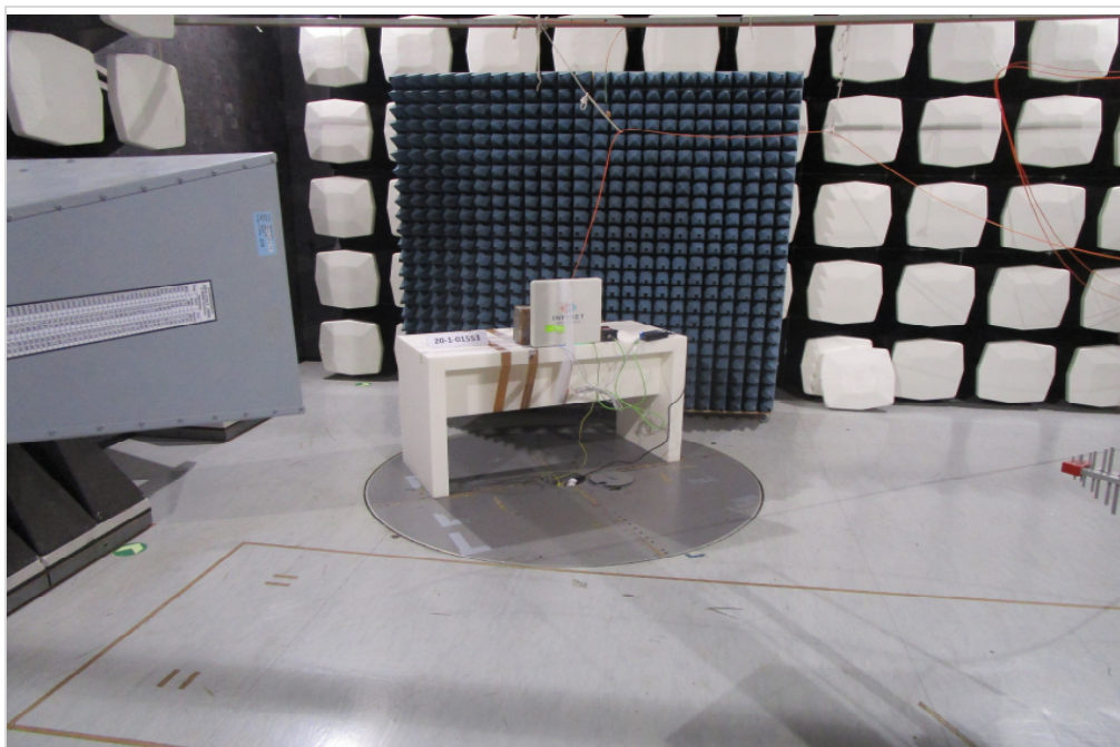
Photograph 2: EUT Test Setup in the semi anechoic chamber, Electric Field Strength
