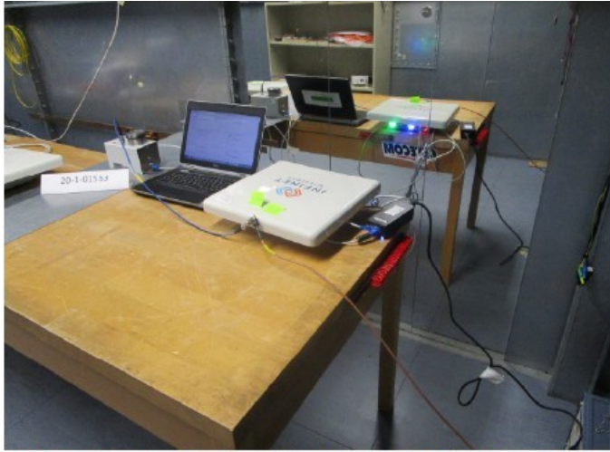
Photograph 4: Conducted emission test set-up , Telecommunication port
