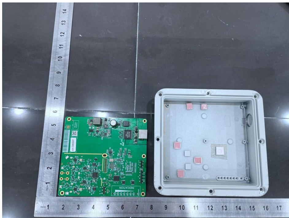
Internal view enclosure of equipment
