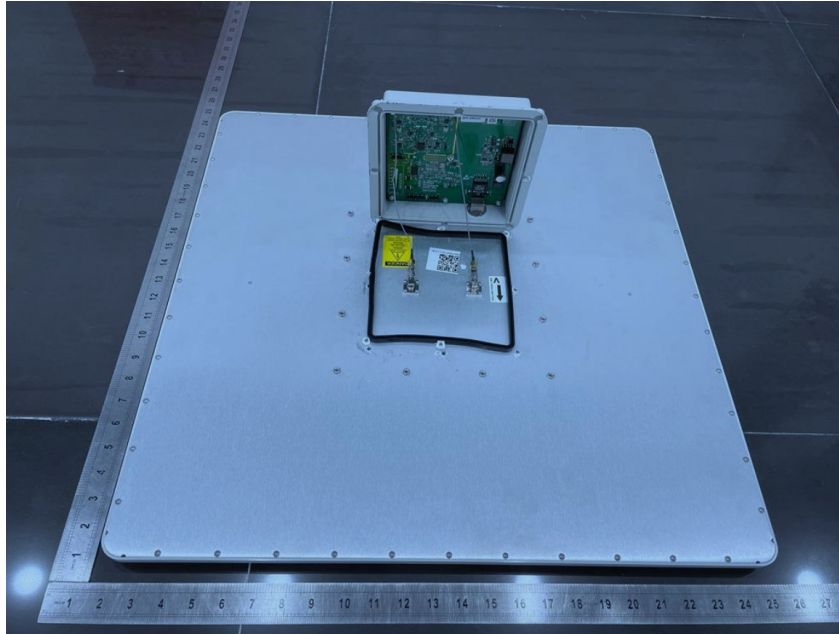
Internal view of E5-STE and cover with two connectors N type
