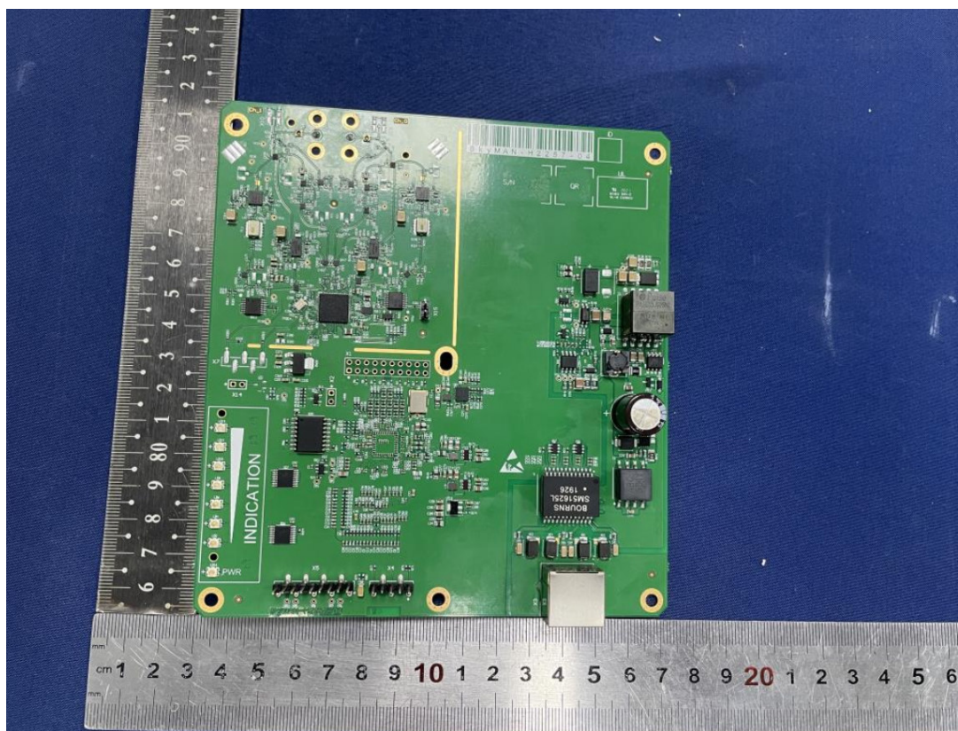
View of main board H2257 with integrated radiomodule
