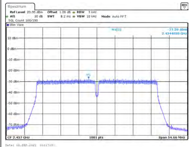
802.11n (40 MHz) / Ant. 0 / 2437 MHz
