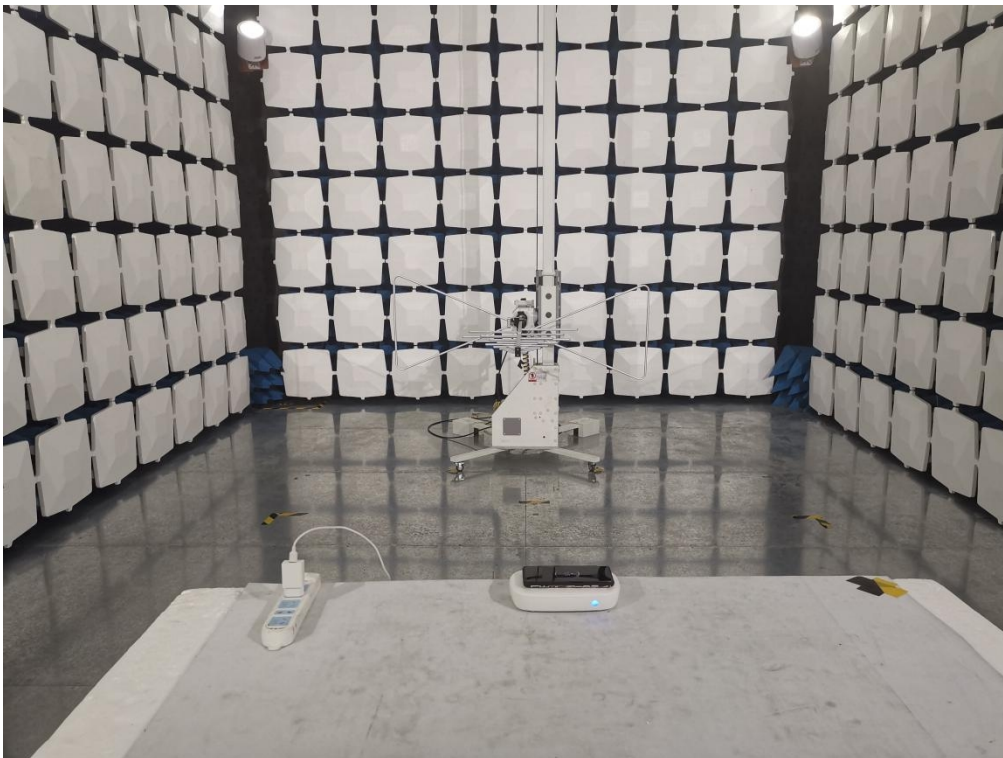
Below 1GHz for radiated emission test setup
