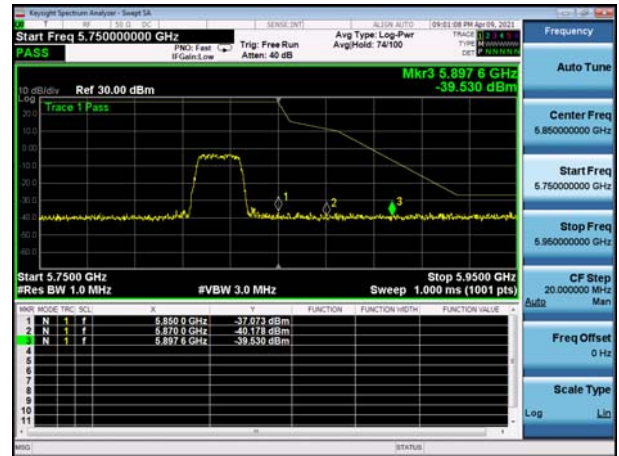
U-NII-3 ,Plot 1,Band Edge-802.11ac(80 MHz),5775MHz,Ant1 Right edge
