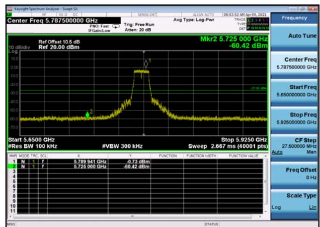
U-NII-3 ,Plot 1,Band Edge-802.11a(20M Hz),5785MHz,Ant0
