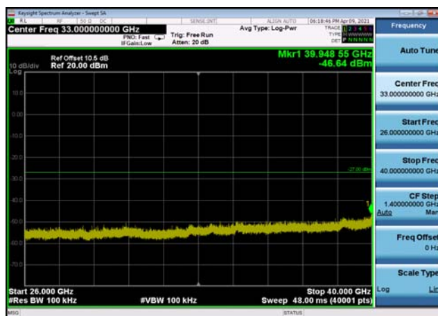
U-NII-3 ,Plot 2,26000MHz~40000MHz-802 .11a(20MHz),5825MHz,Ant1
