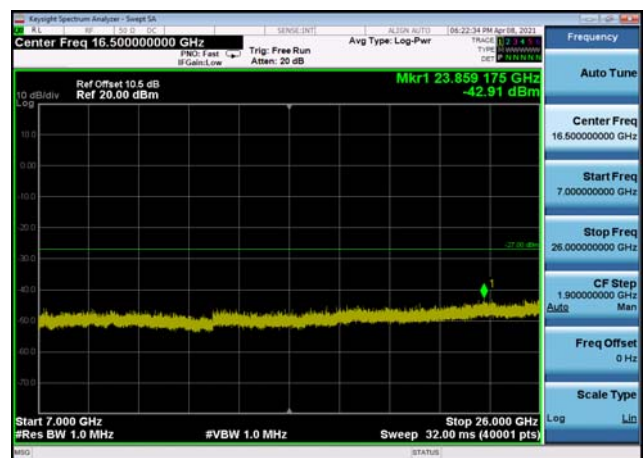
U-NII-3 ,Plot 4,7000MHz~26000MHz-802. 11a(20MHz),5745MHz,Ant1
