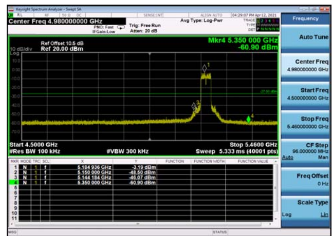
U-NII-1 ,Plot 1,Band Edge-802.11ax(40 MHz),5190MHz,Ant1
