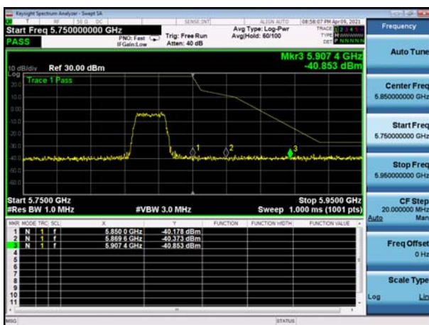
U-NII-3 ,Plot 1,Band Edge-802.11a(20M Hz),5825MHz,Ant0
