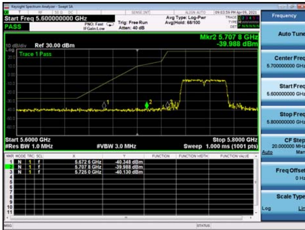
U-NII-3 ,Plot 1,Band Edge-802.11ac(80 MHz),5775MHz,Ant1 left edge
