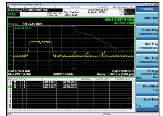
U-NII-3 ,Plot 1,Band Edge-802.11n(40M Hz),5795MHz,Ant1
