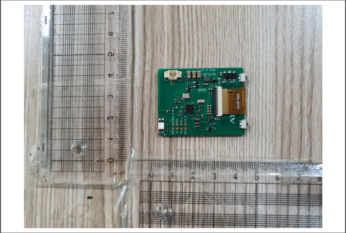
Board-Rear
