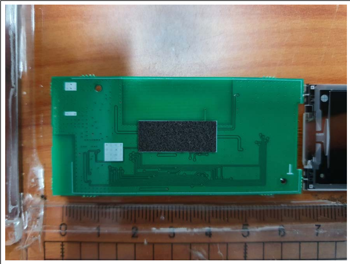
MainBoard-Rear
