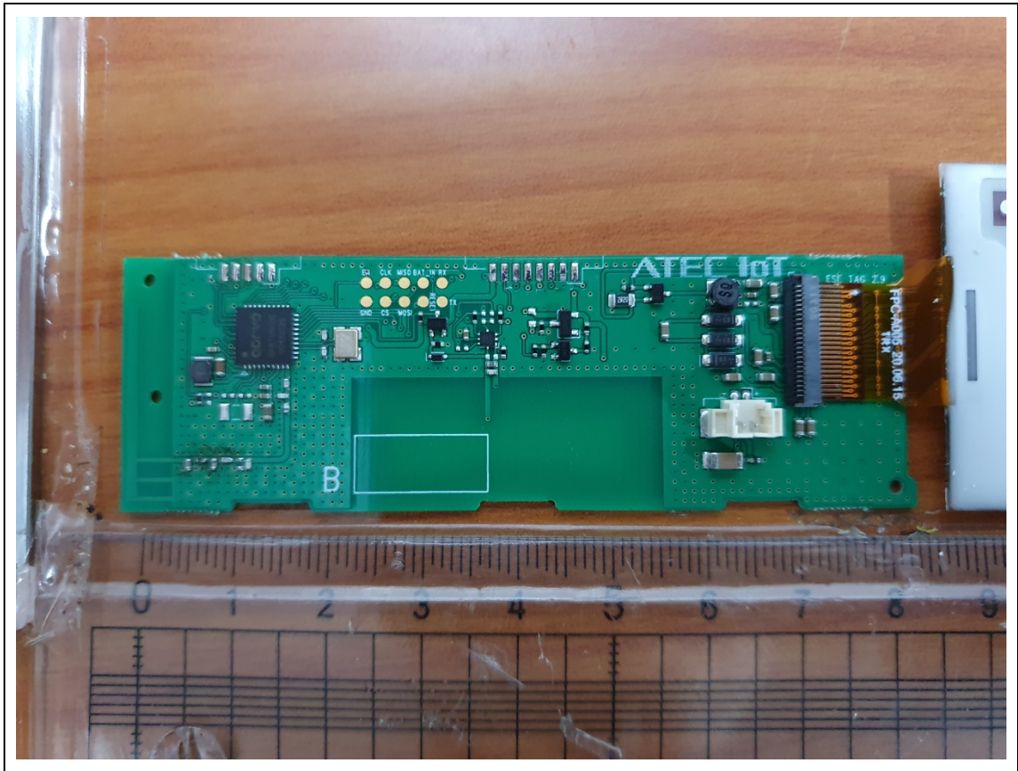
MainBoard-Rear
