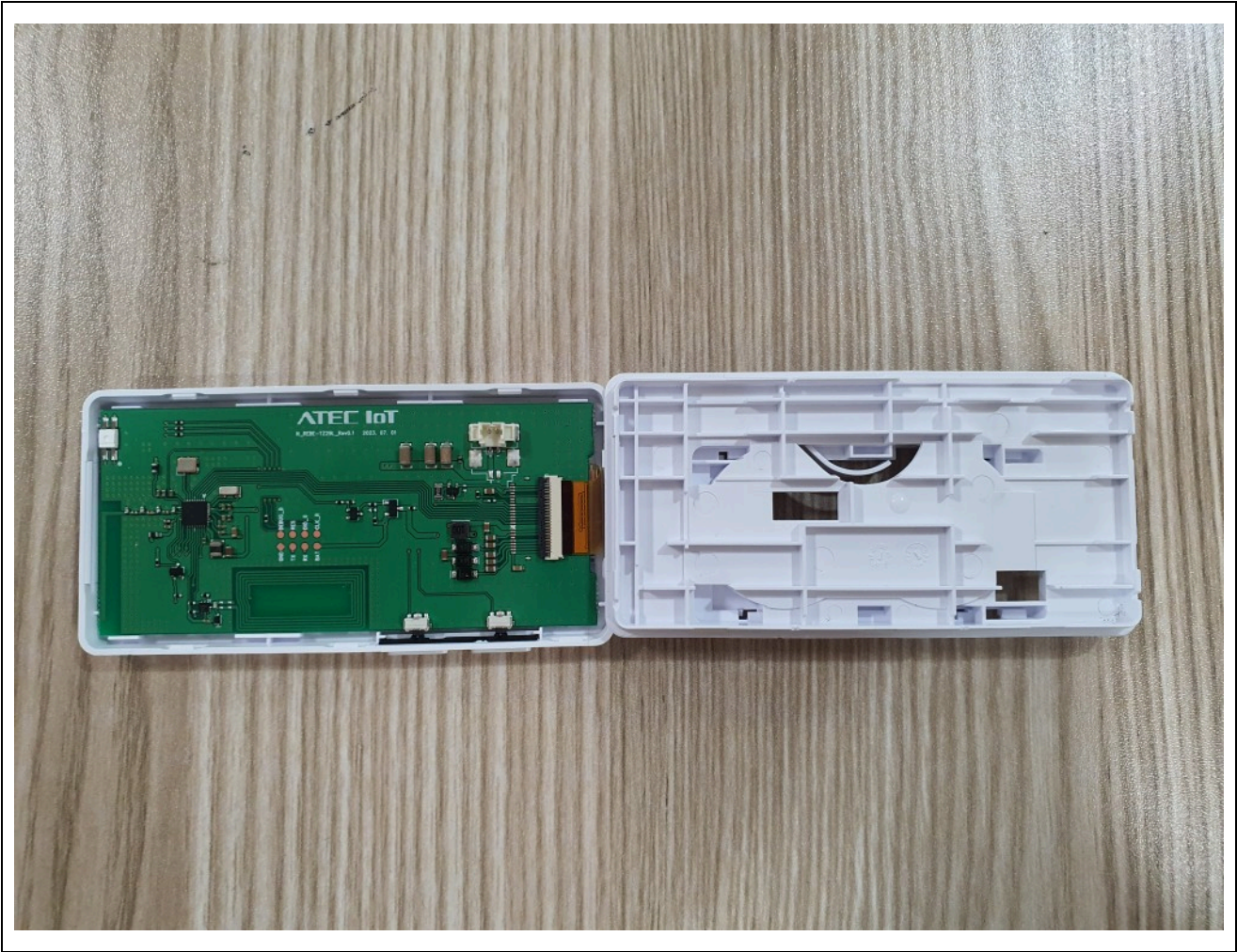
Internal Position
