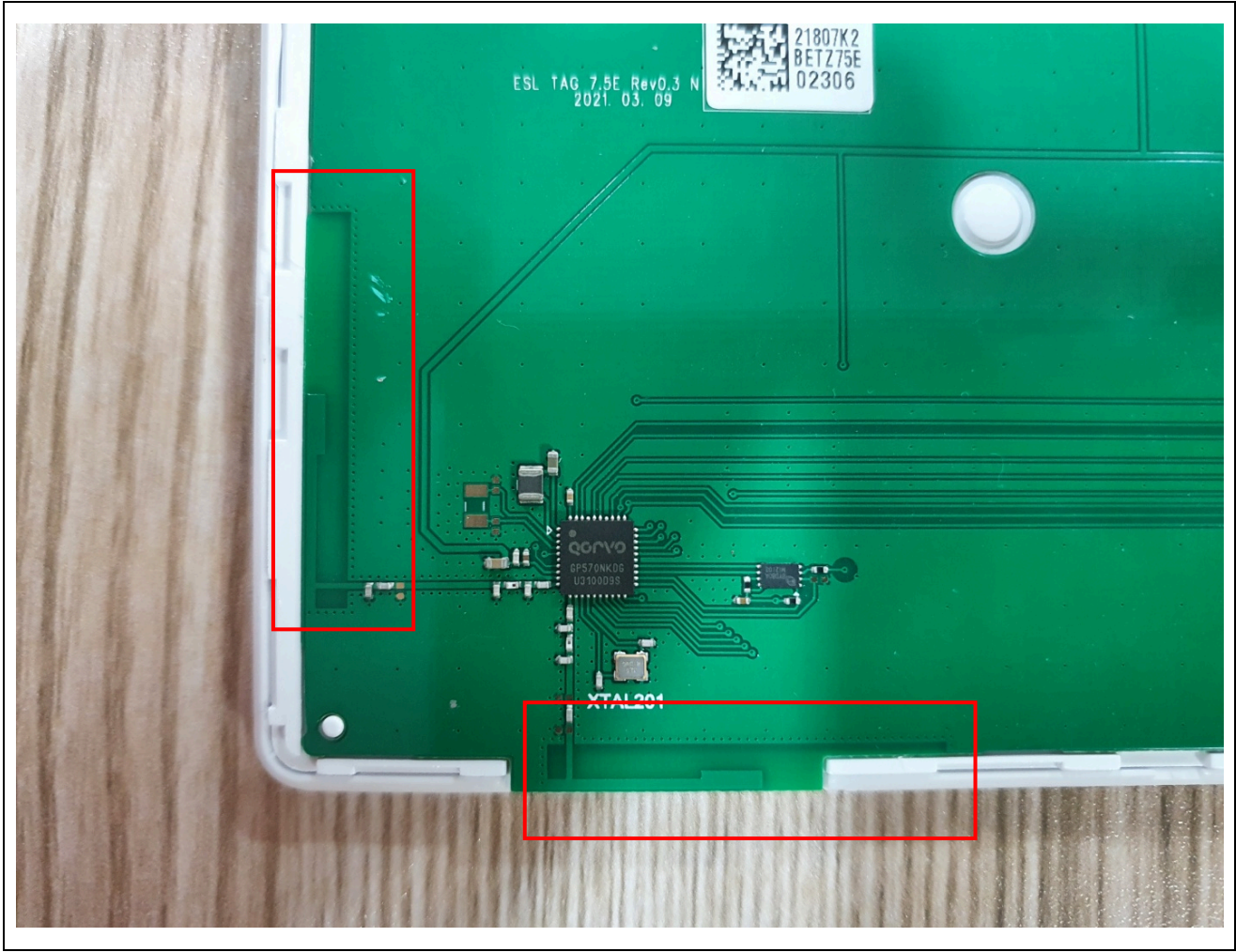
Antenna(2.4GHz ANT)
