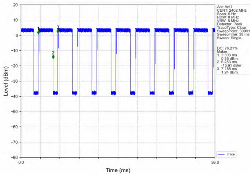
Pi/4DQPSK_2DH5_LCH_2402MHz_Ant1_NTNV
