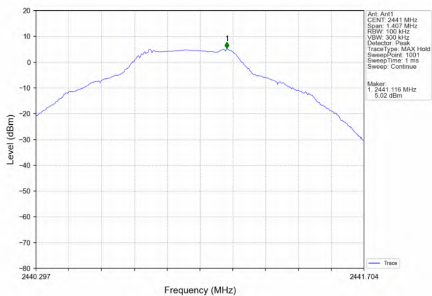
GFSK_DH5_MCH_2441MHz_Ant1_NTNV
