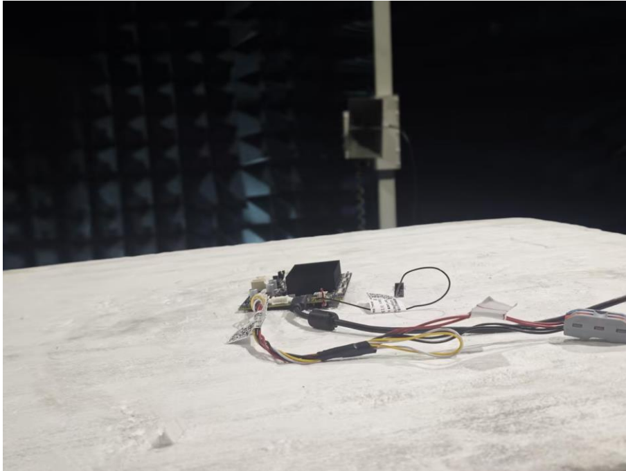
RF Radiated setup (Above 1GHz)
