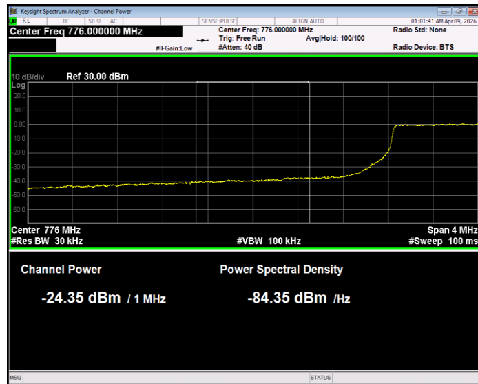
Band13 QPSK BW=5MHz Channel=23255 RB Size=1 Position=#0 Normal
