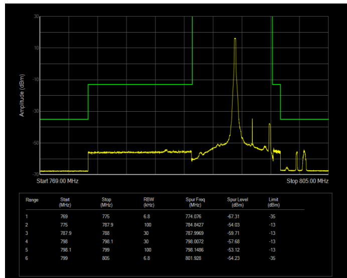
Band14 QPSK BW=5MHz Channel=23355 RB Size=1 Position=#0 Extended
