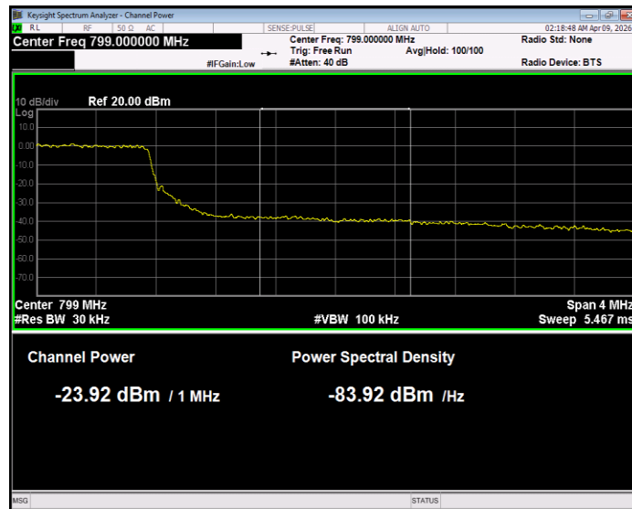
Band14 QPSK BW=10MHz Channel=23330 RB Size=1 Position=#0 Normal
