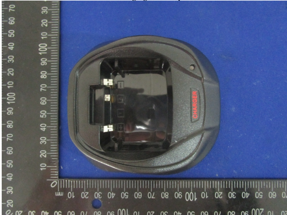
EUT – Charging Base Top View
