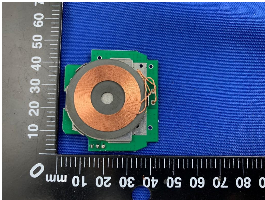
SUB BOARD REAR VIEW (WITH SHIELDING)
