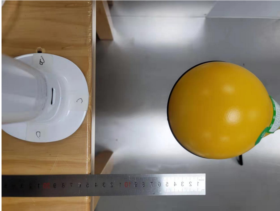
H-field Test Setup Photo of Position C(15cm)
