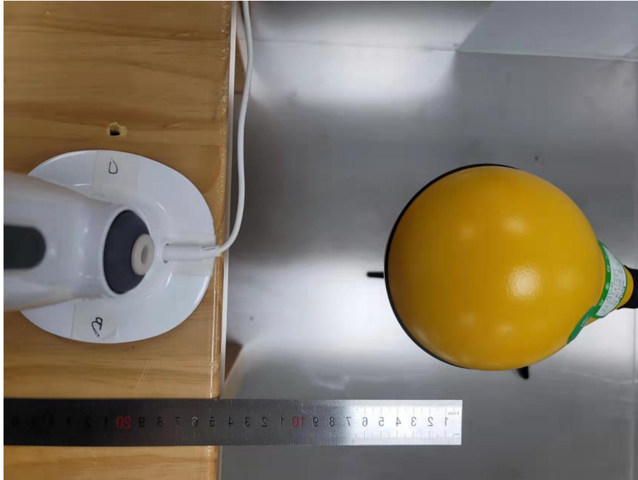
H-field Test Setup Photo of Position A(15cm)
