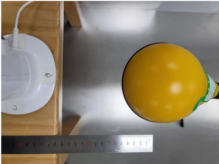
H-field Test Setup Photo of Position B(15cm)
