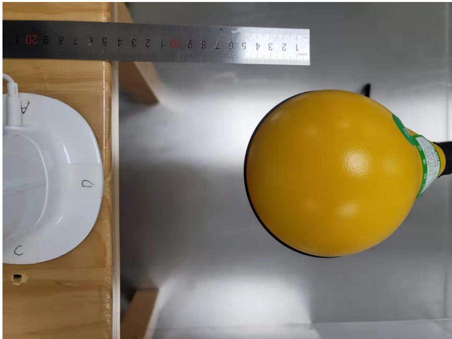
H-field Test Setup Photo of Position D(15cm)
