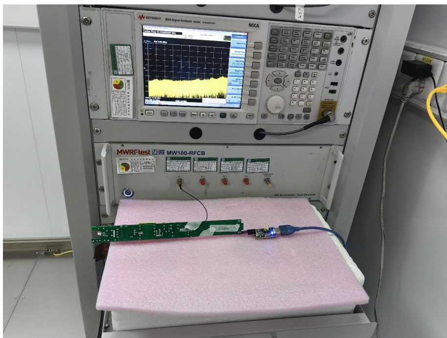
RF Conduction Measurement Photos
