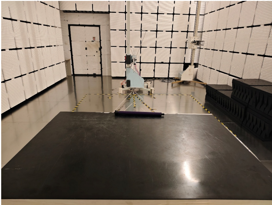
Radiated Emission Measurement Photos
