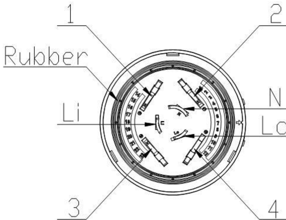
Figure 3: Bottom view
