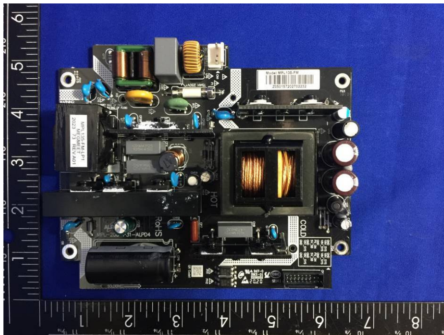
EUT Housing and Board View 12
