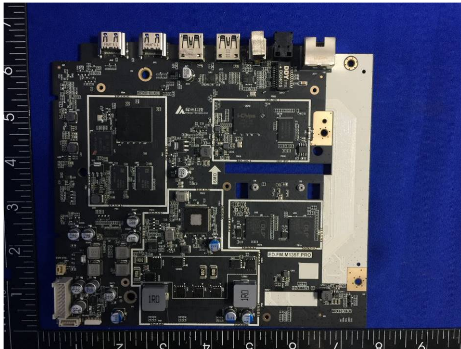
EUT Housing and Board View 11
