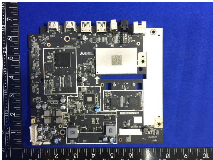
EUT Housing and Board View 10
