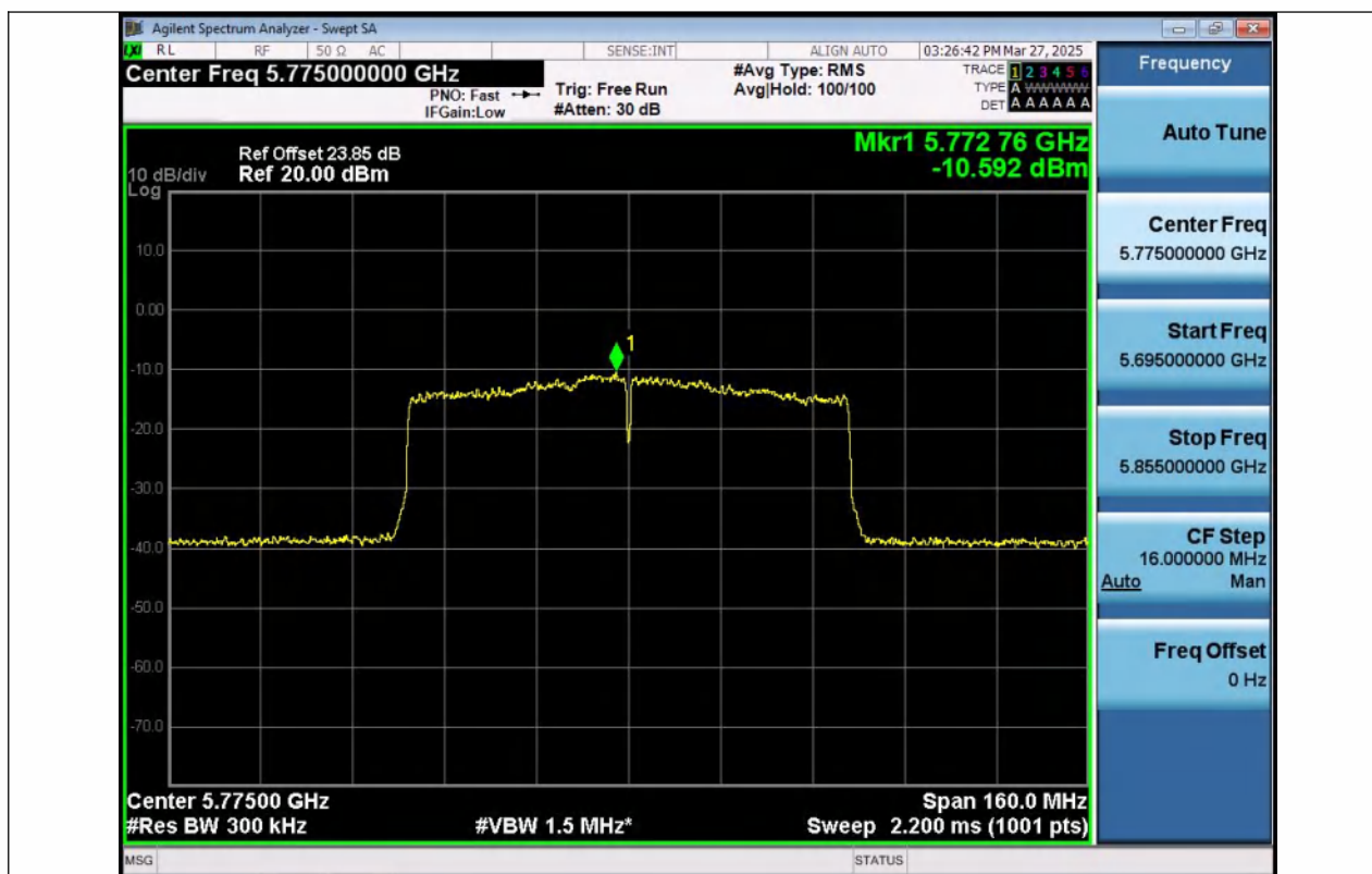
11AC80MIMO-Ant1-5775-PASS
