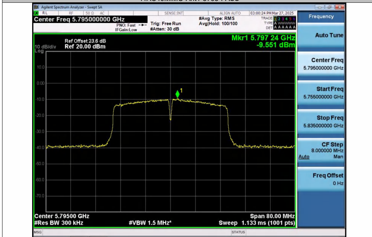
11AC40MIMO-Ant2-5795-PASS
