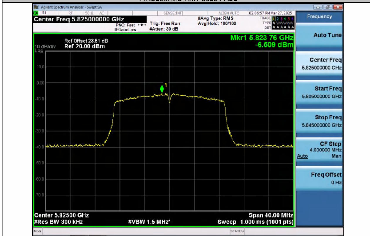
11AC20MIMO-Ant2-5825-PASS
