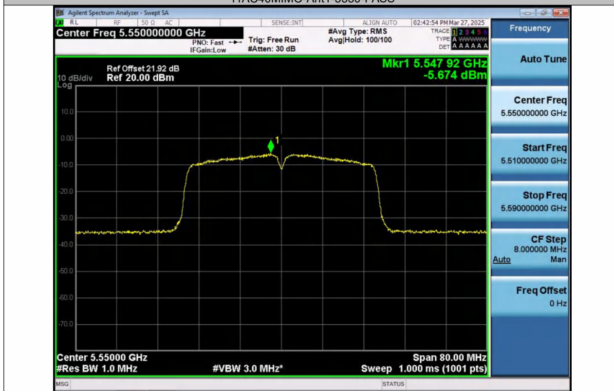
11AC40MIMO-Ant2-5550-PASS
