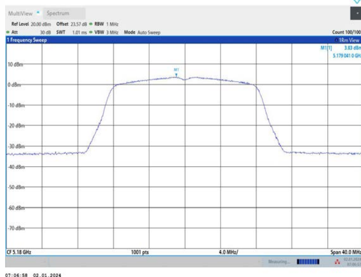
11A_Ant2_5180
