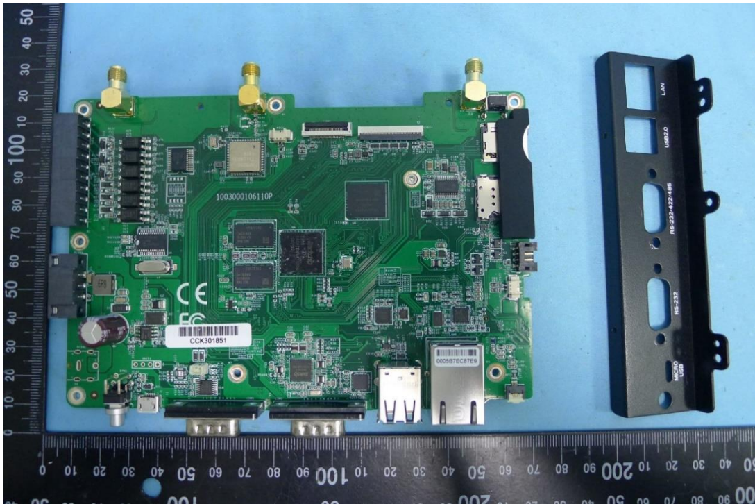
(7) EUT Photo
