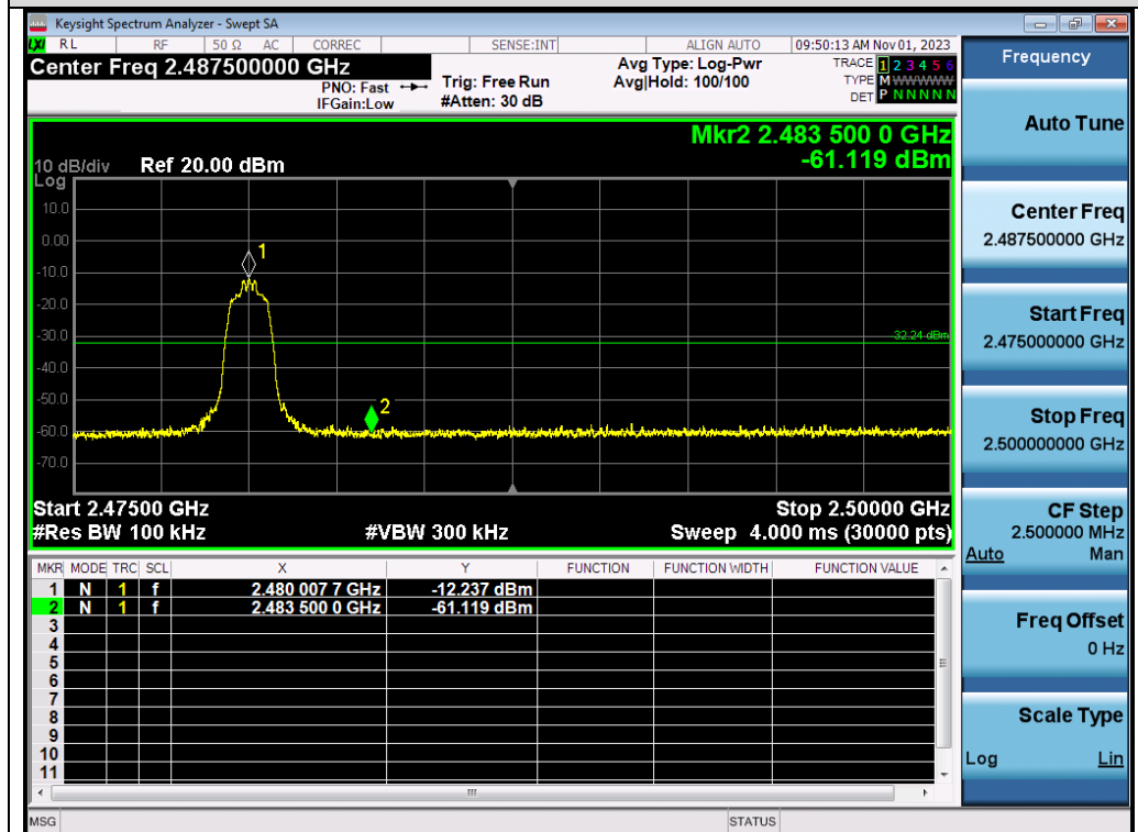
Test_Graph_π /4-DQPSK_ANT1_2480_Higher Band Edge Emissions
