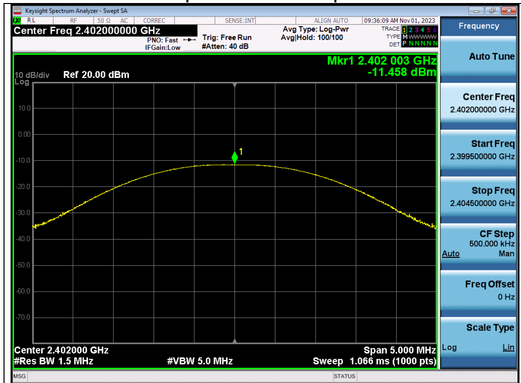
Test_Graph_GFSK_ANT1_2402_Peak Power
