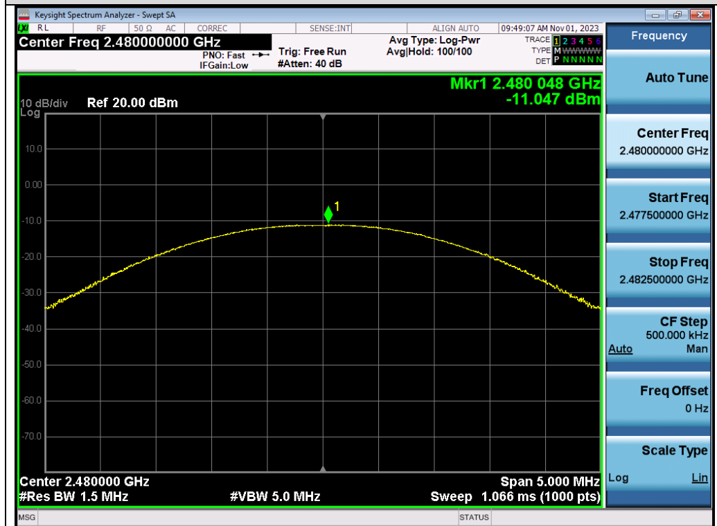
Test_Graph_π /4-DQPSK_ANT1_2480_Peak Power
