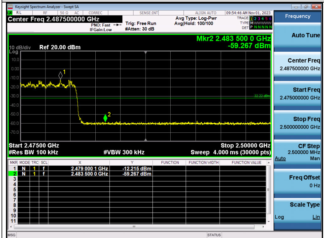
Test_Graph_π /4-DQPSK_HOP_ANT1_NA_Higher Band Edge Emissions
