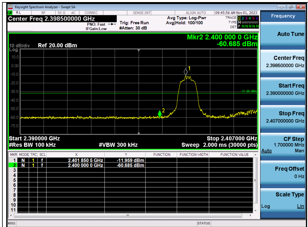
Test_Graph_π /4-DQPSK_ANT1_2402_Lower Band Edge Emissions
