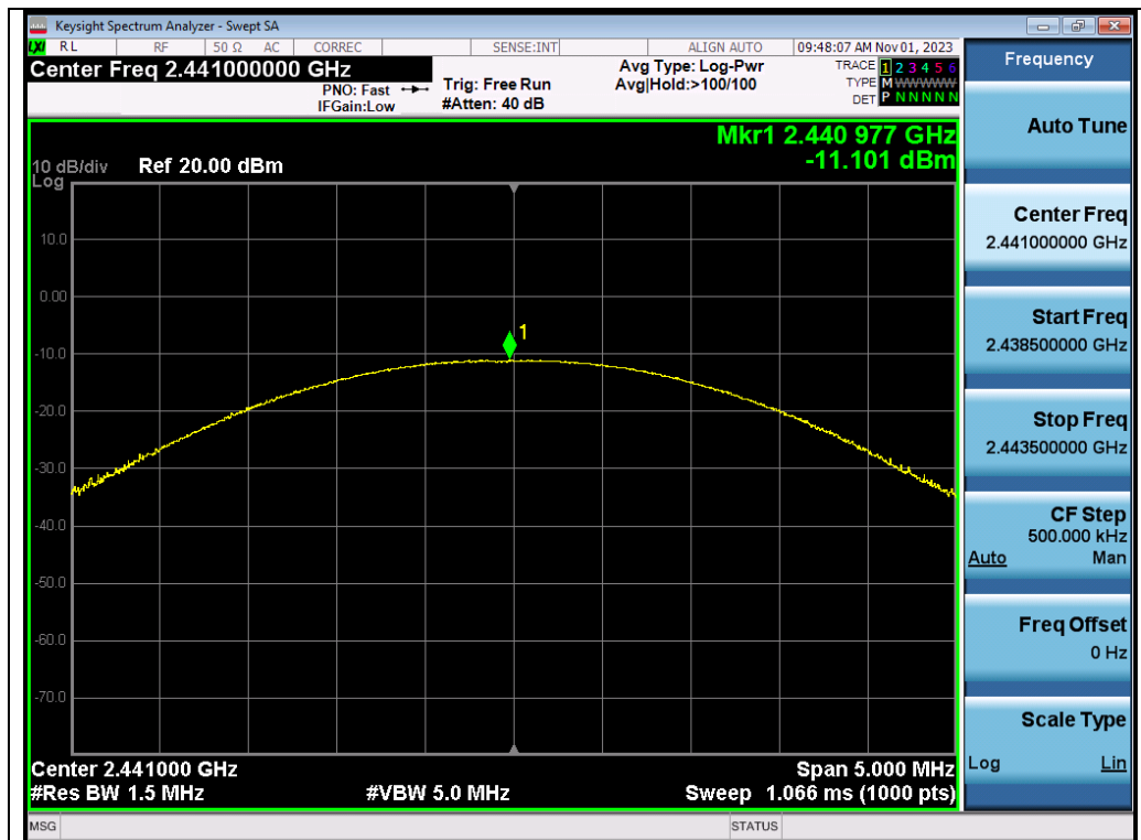
Test_Graph_π /4-DQPSK_ANT1_2441_Peak Power
