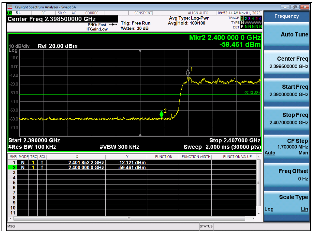
Test_Graph_π /4-DQPSK_HOP_ANT1_NA_Lower Band Edge Emissions
