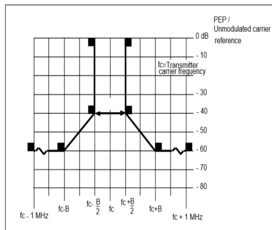
Figure 5: Spectral mask for digital systems above 1 GHz, normalized to channel bandwidth B
