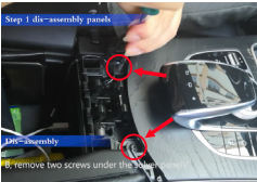
2. Remove the two screws under the silver panel
