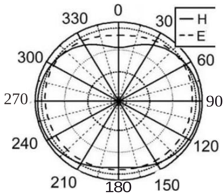
27.145 MHZ radiation patter
