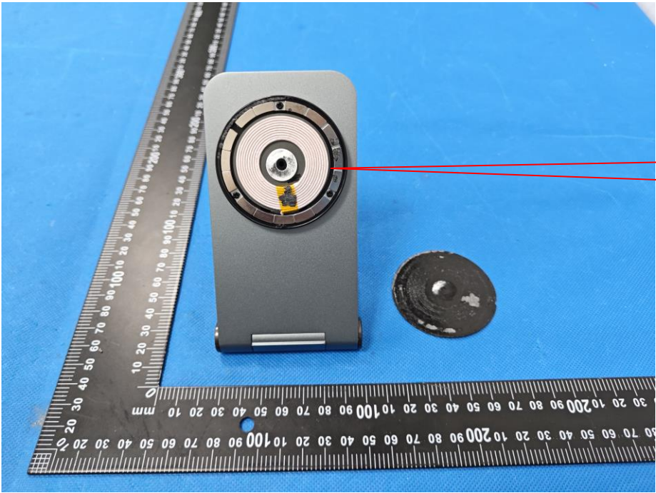
Phone Antenna
