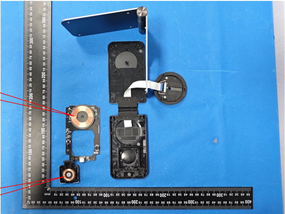
Earphone Antenna
