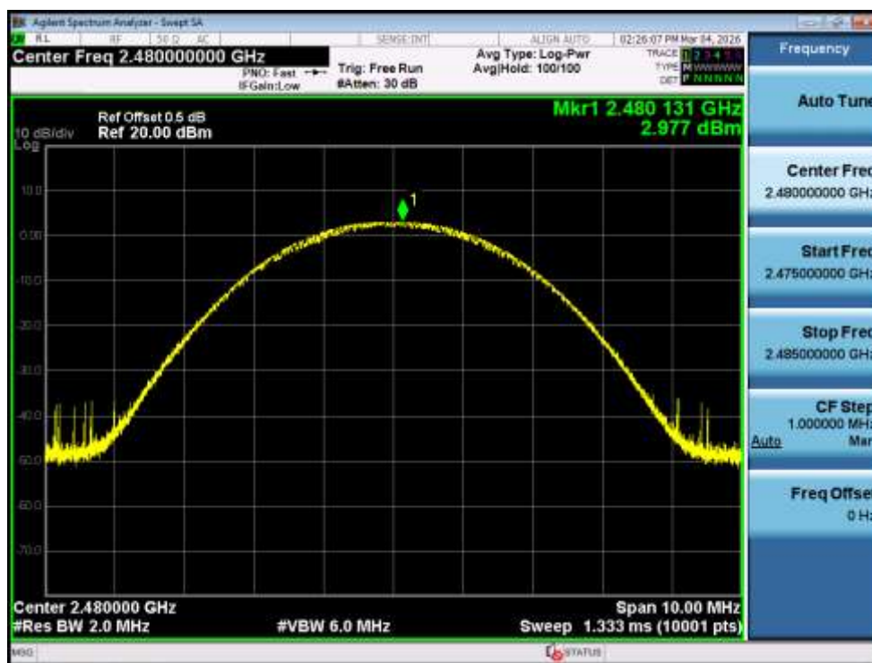
Power NVNT 2-DH5 2480MHz
