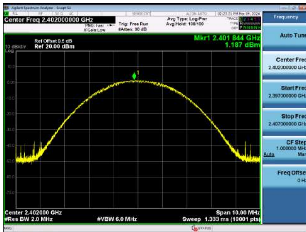
Power NVNT 2-DH5 2402MHz
