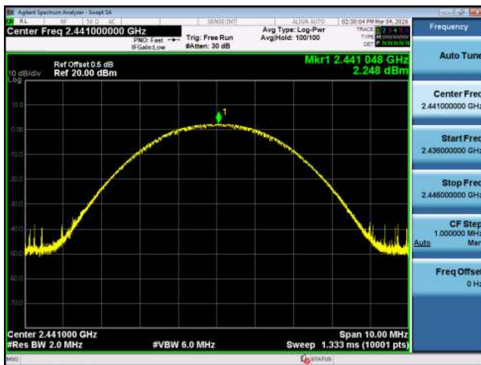
Power NVNT 3-DH5 2441MHz
