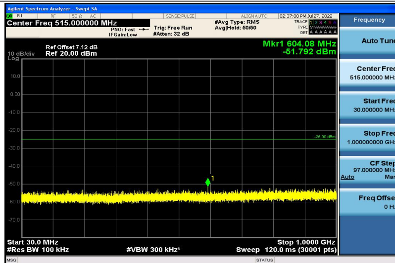
Band7-15MHz-16QAM-21100-1RB#0-30~1000MHz
