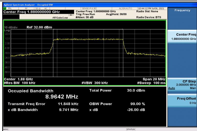
Band2-10MHz-16QAM-18900-50RB#0-8.9642
