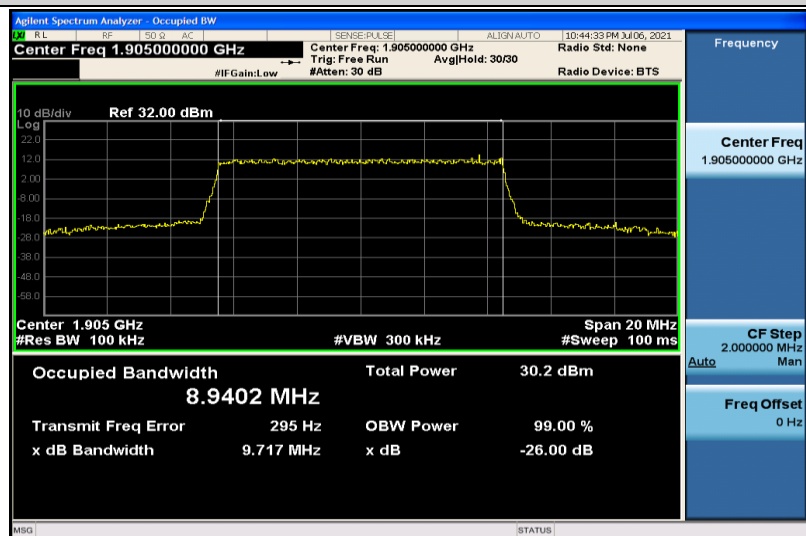
Band2-10MHz-16QAM-19150-50RB#0-8.9402
