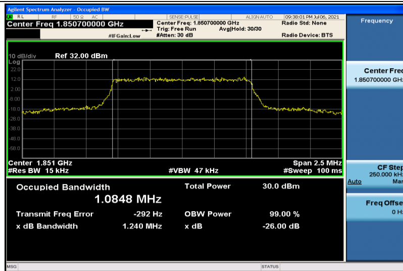
Band2-1.4MHz-QPSK-18607-6RB#0-1.0848
