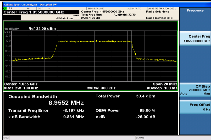
Band2-10MHz-16QAM-18650-50RB#0-8.9552
