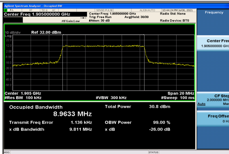
Band2-10MHz-QPSK-19150-50RB#0-8.9633
