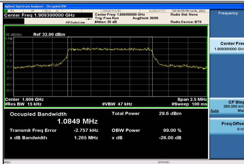
Band2-1.4MHz-QPSK-19193-6RB#0-1.0849
