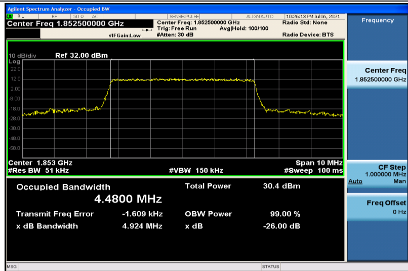
Band2-5MHz-16QAM-18625-25RB#0-4.4800
