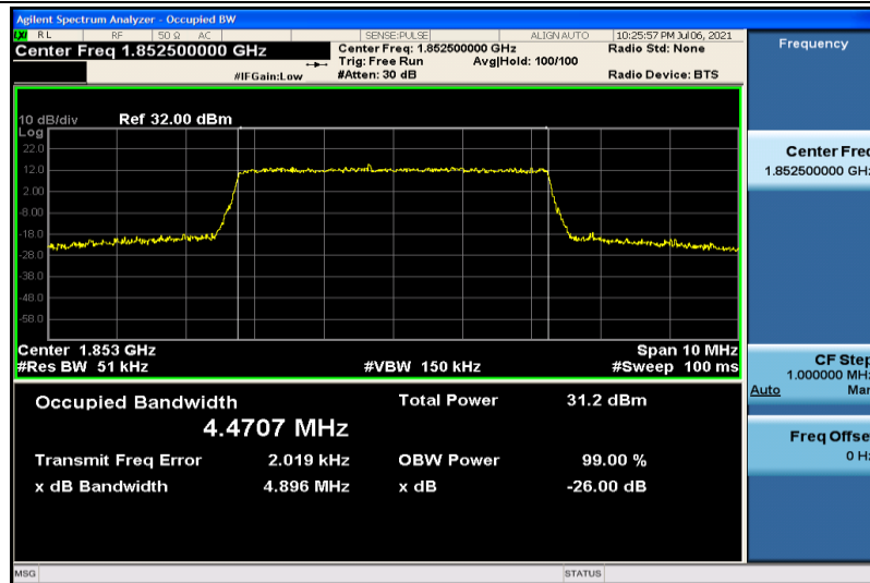
Band2-5MHz-QPSK-18625-25RB#0-4.4707
