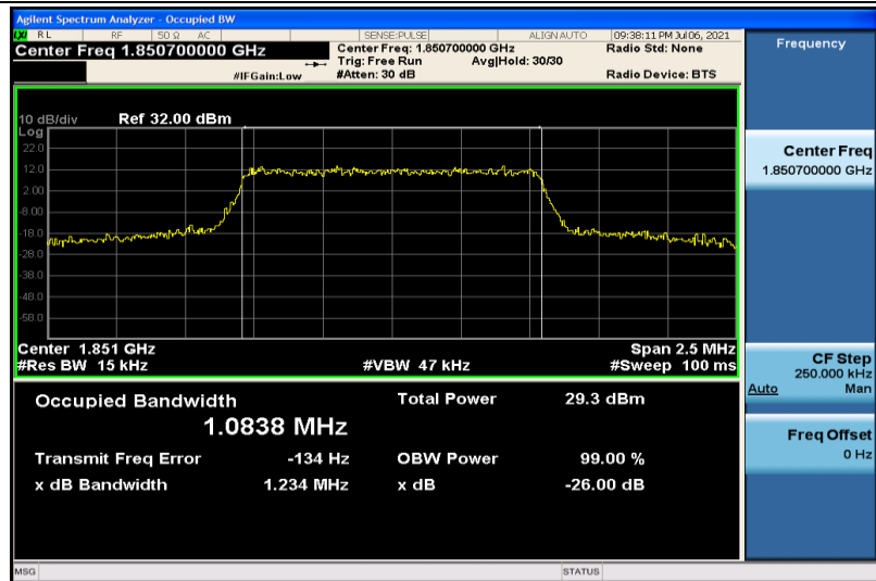
Band2-1.4MHz-16QAM-18607-6RB#0-1.0838
