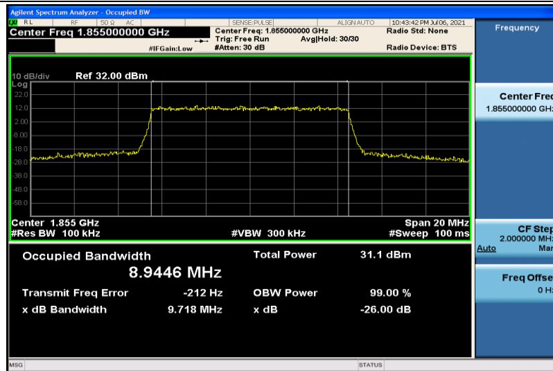
Band2-10MHz-QPSK-18650-50RB#0-8.9446
