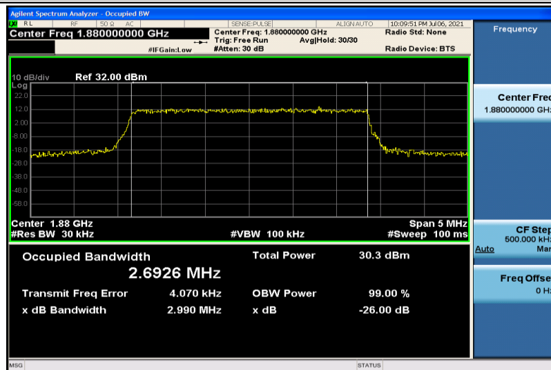
Band2-3MHz-QPSK-18900-15RB#0-2.6926
