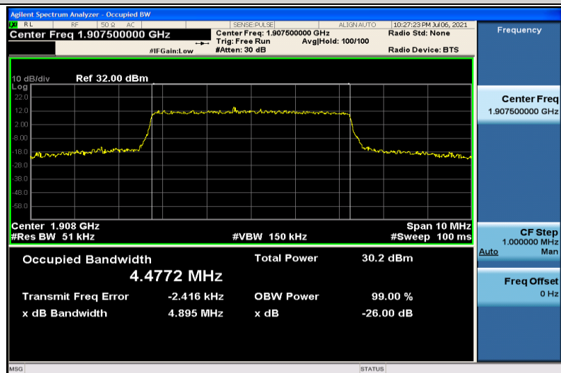
Band2-5MHz-16QAM-19175-25RB#0-4.4772
