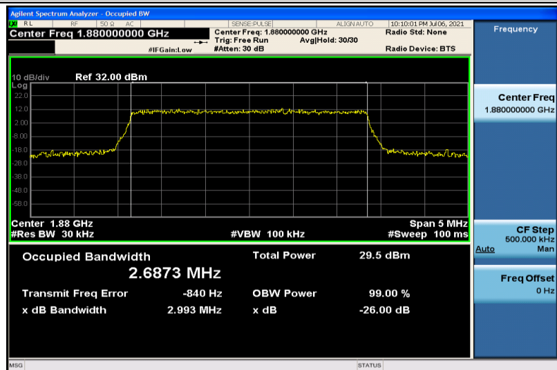
Band2-3MHz-16QAM-18900-15RB#0-2.6873
