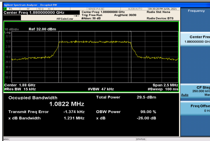
Band2-1.4MHz-QPSK-18900-6RB#0-1.0822
