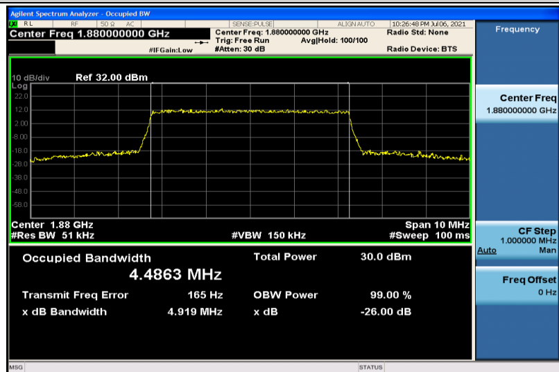
Band2-5MHz-16QAM-18900-25RB#0-4.4863
