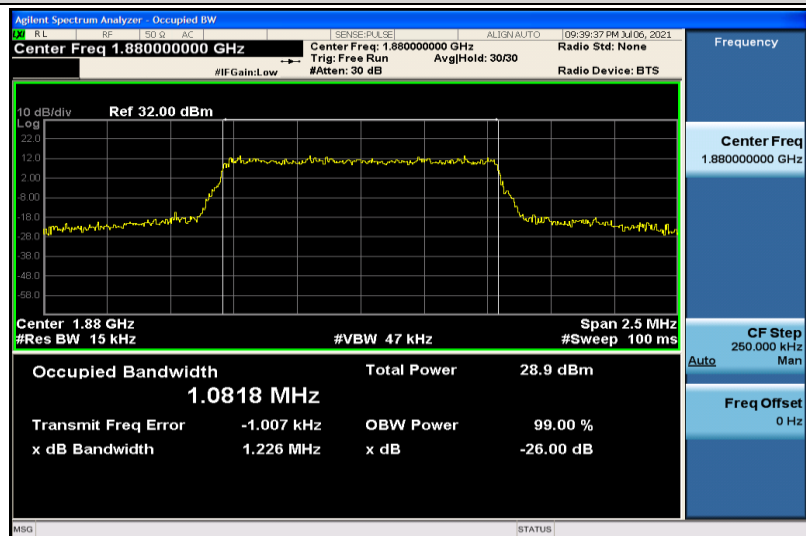
Band2-1.4MHz-16QAM-18900-6RB#0-1.0818
