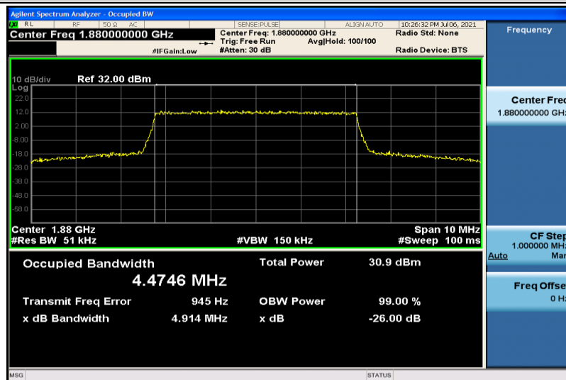
Band2-5MHz-QPSK-18900-25RB#0-4.4746
