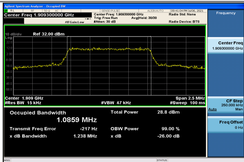
Band2-1.4MHz-16QAM-19193-6RB#0-1.0859
