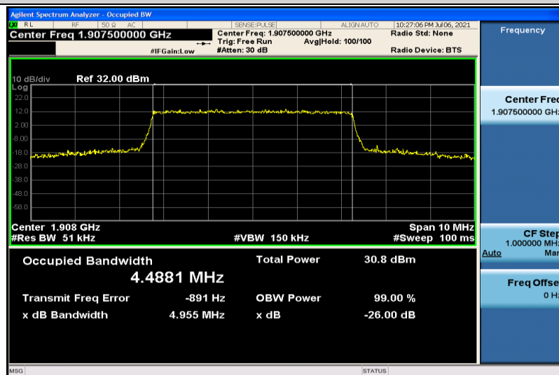
Band2-5MHz-QPSK-19175-25RB#0-4.4881
