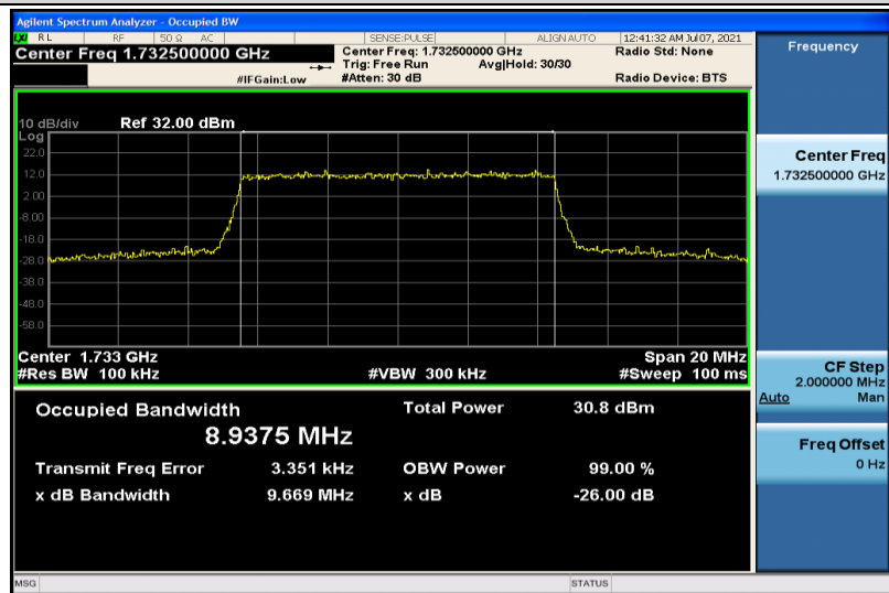
Band4-10MHz-QPSK-20175-50RB#0-8.9375
