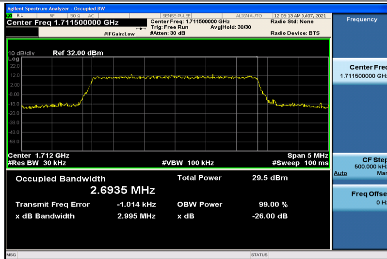
Band4-3MHz-16QAM-19965-15RB#0-2.6935
