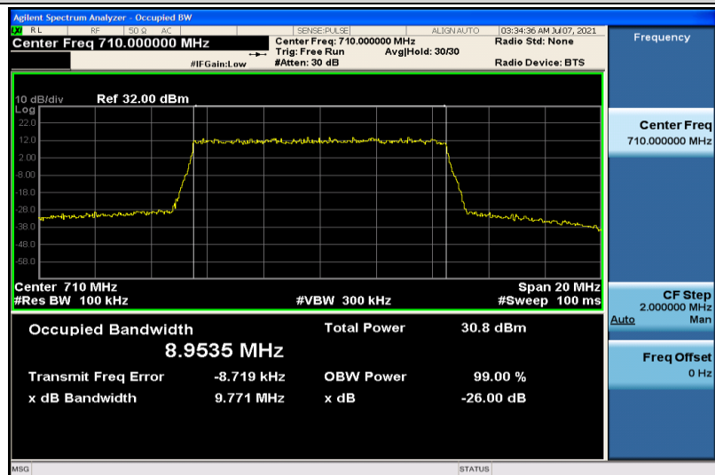
Band17-10MHz-QPSK-23790-50RB#0-8.9535
