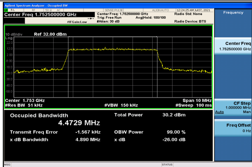
Band4-5MHz-16QAM-20375-25RB#0-4.4729
