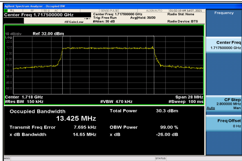
Band4-15MHz-16QAM-20025-75RB#0-13.425
