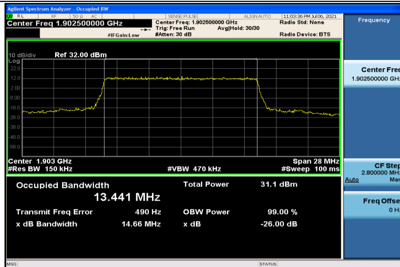
Band2-15MHz-QPSK-19125-75RB#0-13.441
