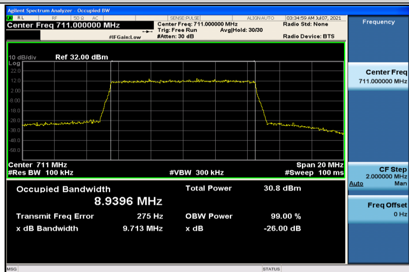
Band17-10MHz-QPSK-23800-50RB#0-8.9396
