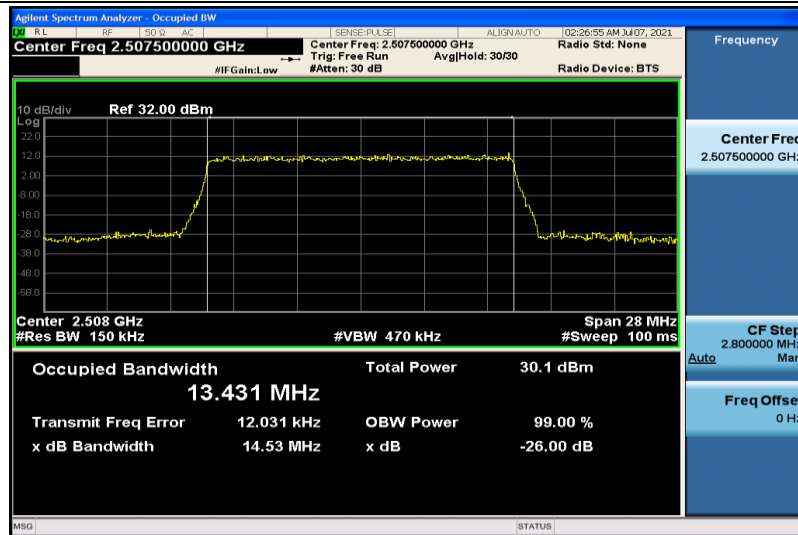
Band7-15MHz-16QAM-20825-75RB#0-13.431
