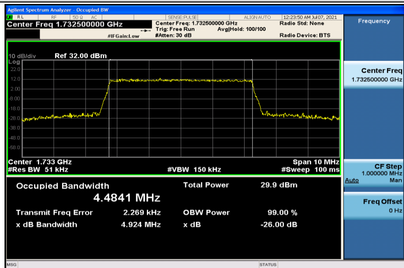
Band4-5MHz-16QAM-20175-25RB#0-4.4841
