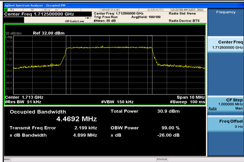
Band4-5MHz-QPSK-19975-25RB#0-4.4692
