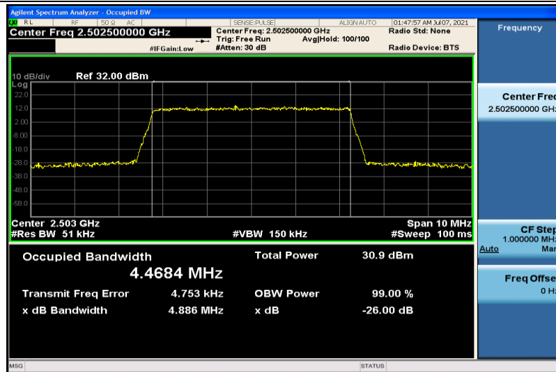
Band7-5MHz-QPSK-20775-25RB#0-4.4684
