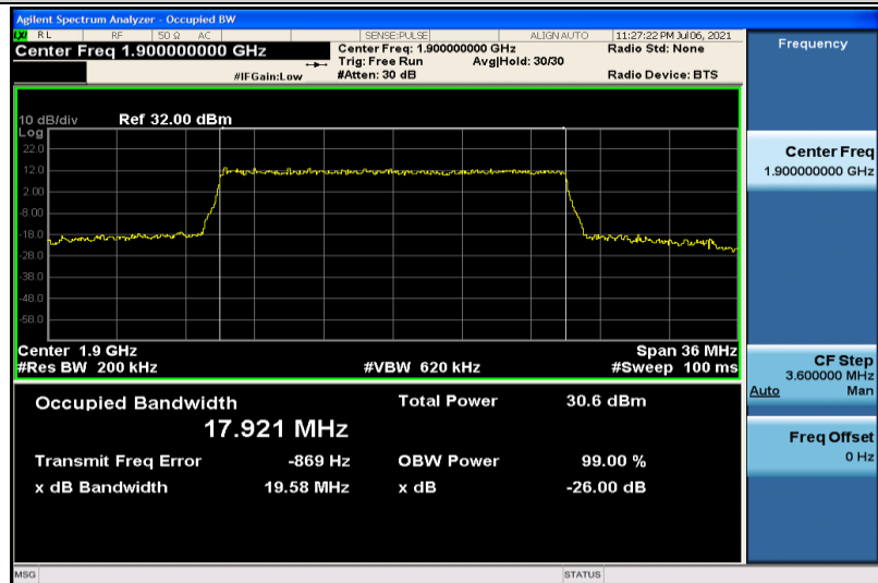
Band2-20MHz-16QAM-19100-100RB#0-17.921
