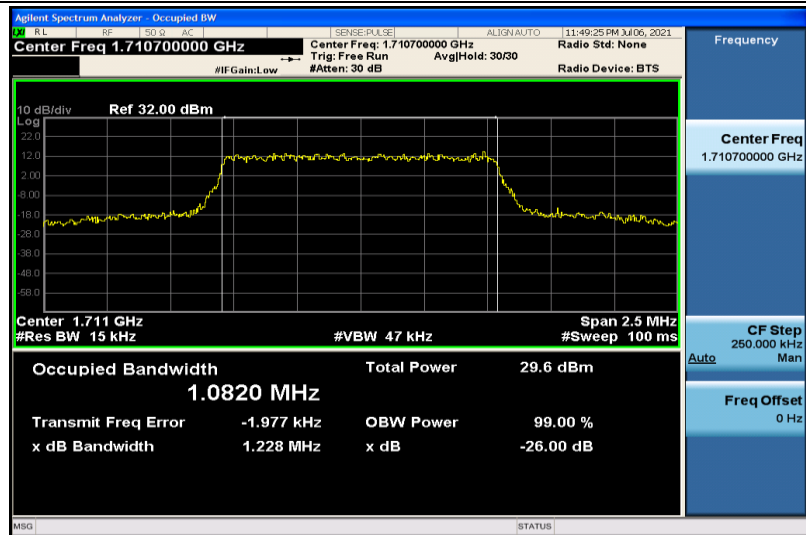
Band4-1.4MHz-QPSK-19957-6RB#0-1.0820
