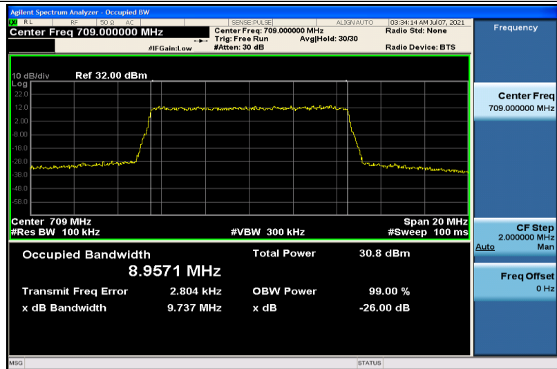
Band17-10MHz-QPSK-23780-50RB#0-8.9571
