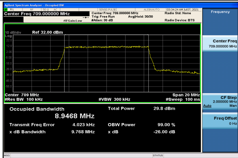
Band17-10MHz-16QAM-23780-50RB#0-8.9468
