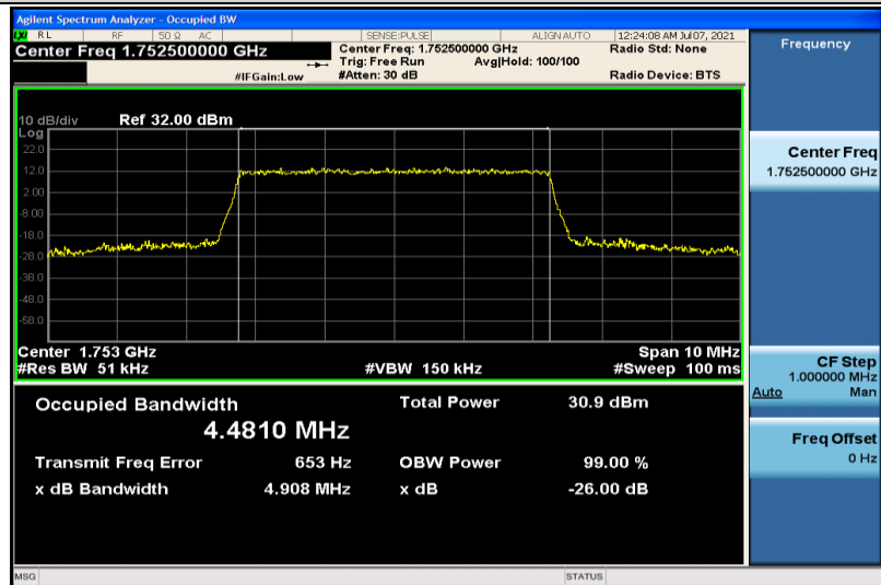
Band4-5MHz-QPSK-20375-25RB#0-4.4810
