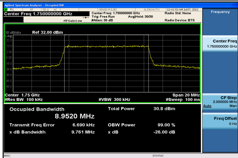
Band4-10MHz-QPSK-20350-50RB#0-8.9520
