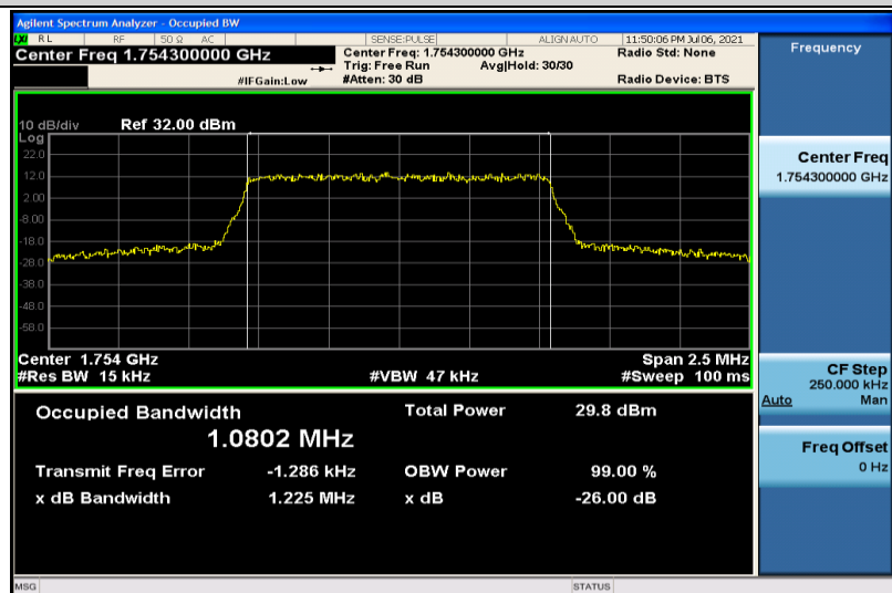
Band4-1.4MHz-QPSK-20393-6RB#0-1.0802
