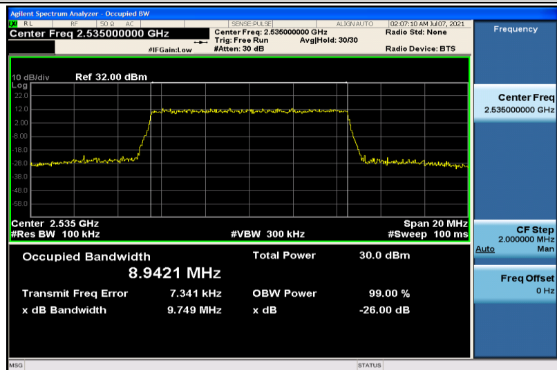
Band7-10MHz-16QAM-21100-50RB#0-8.9421
