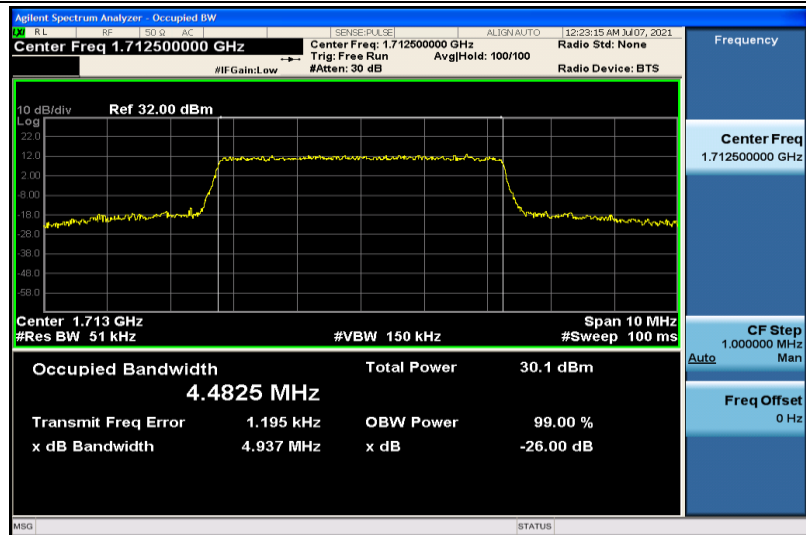
Band4-5MHz-16QAM-19975-25RB#0-4.4825
