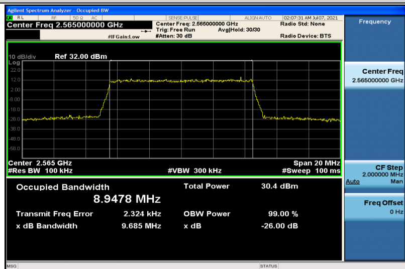
Band7-10MHz-16QAM-21400-50RB#0-8.9478
