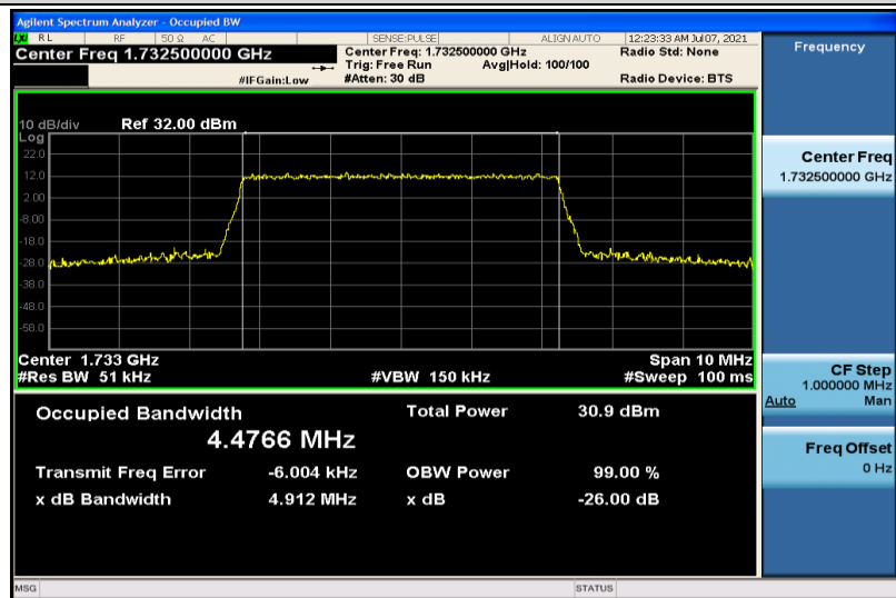
Band4-5MHz-QPSK-20175-25RB#0-4.4766
