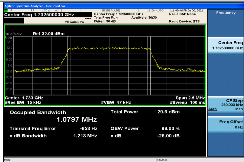
Band4-1.4MHz-QPSK-20175-6RB#0-1.0797
